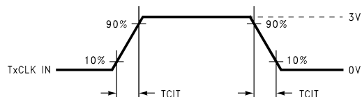
Figure 8. DS90C363 (Transmitter) Input Clock Transition Time
