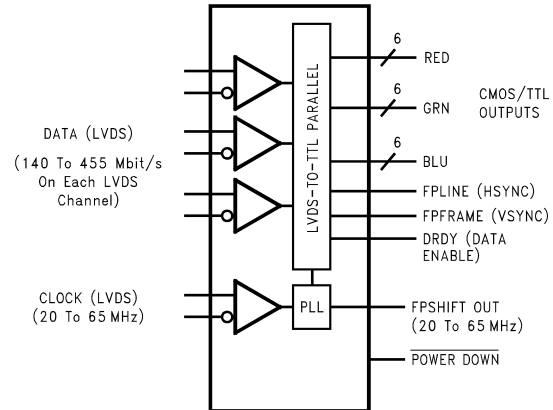
Figure 3. DS90CF364
