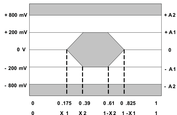
Figure 4-5. OBSAI TX Output Mask for Rates \leq 3.072 Gbps
