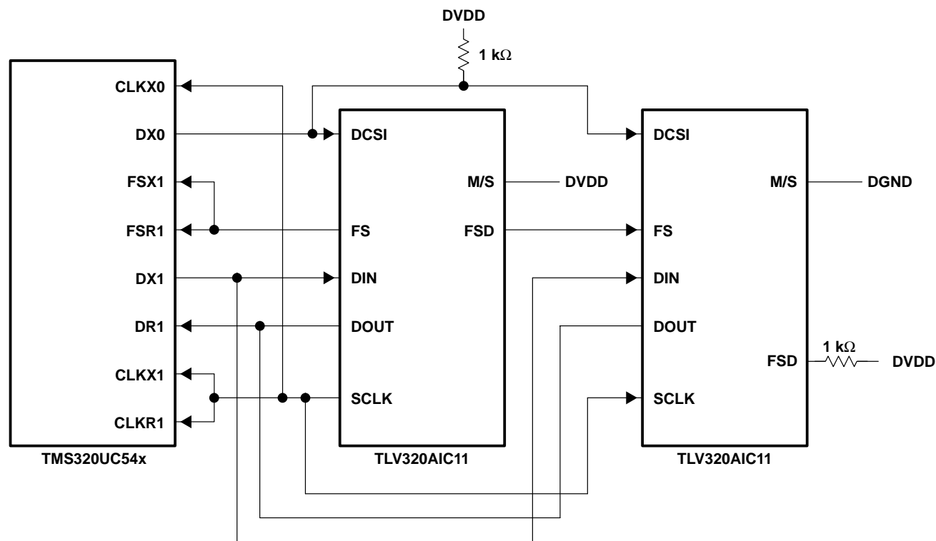
Figure 3–8. Direct Configuration
