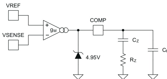
Figure 7-3. Transconductance Error Amplifier With Typical Compensation Network
