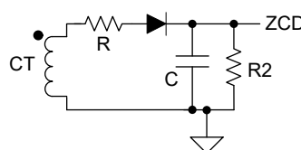
Figure 7-2. More Accurate Time Delay Circuit
