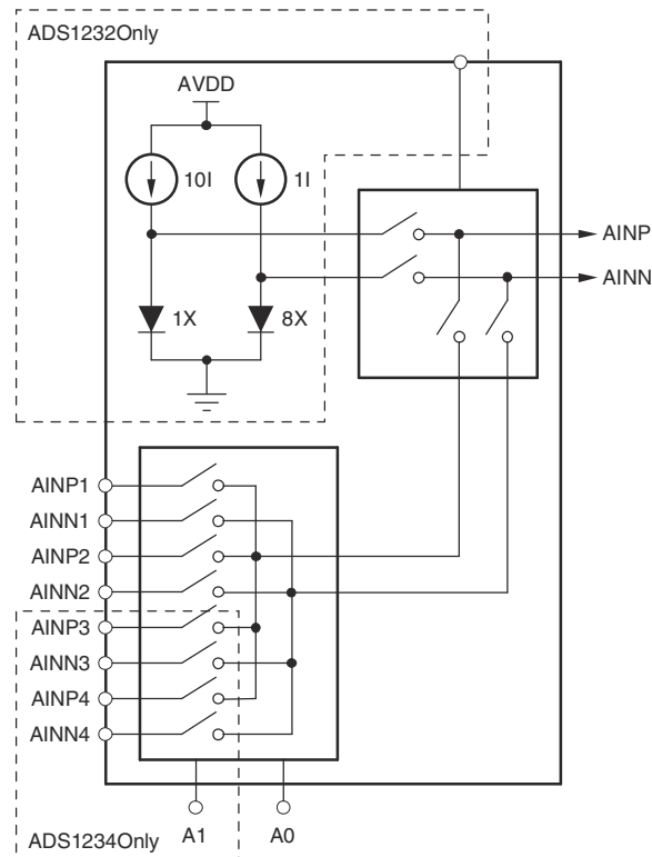
Figure 8-1. Measurement of the Temperature Sensor in the Input Multiplexer
