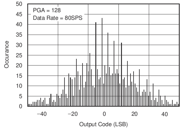
Figure 6-8. Noise Histogram
