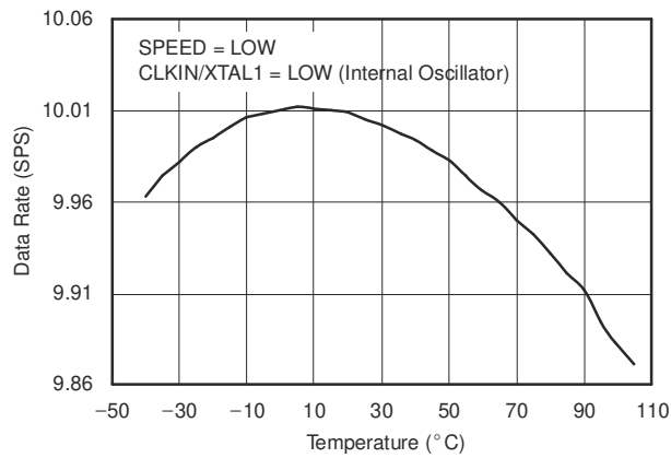
Figure 6-25. Data Rate vs Temperature
