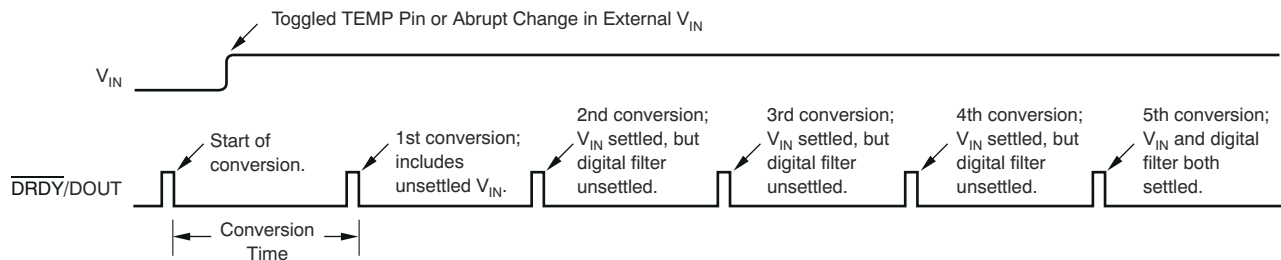
Figure 8-8. Settling Time in Continuous Conversion Mode
