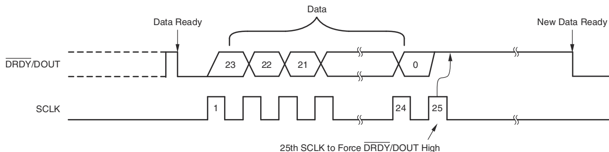
Figure 8-10. Data Retrieval With \overline{\text{DRDY}}/\text{DOUT} Forced High Afterwards
