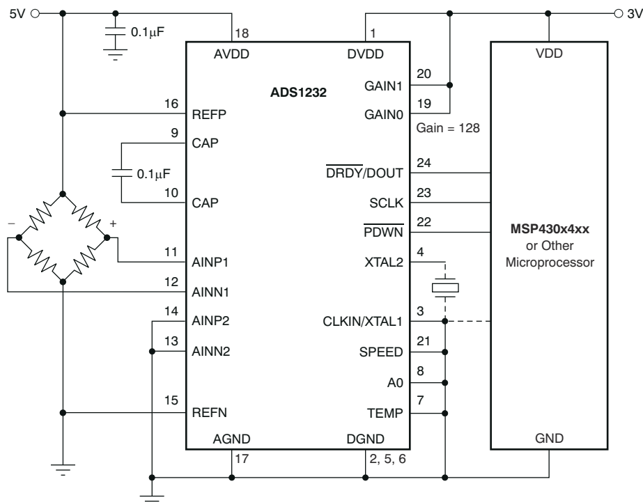
Figure 9-1. Weigh-Scale Application
