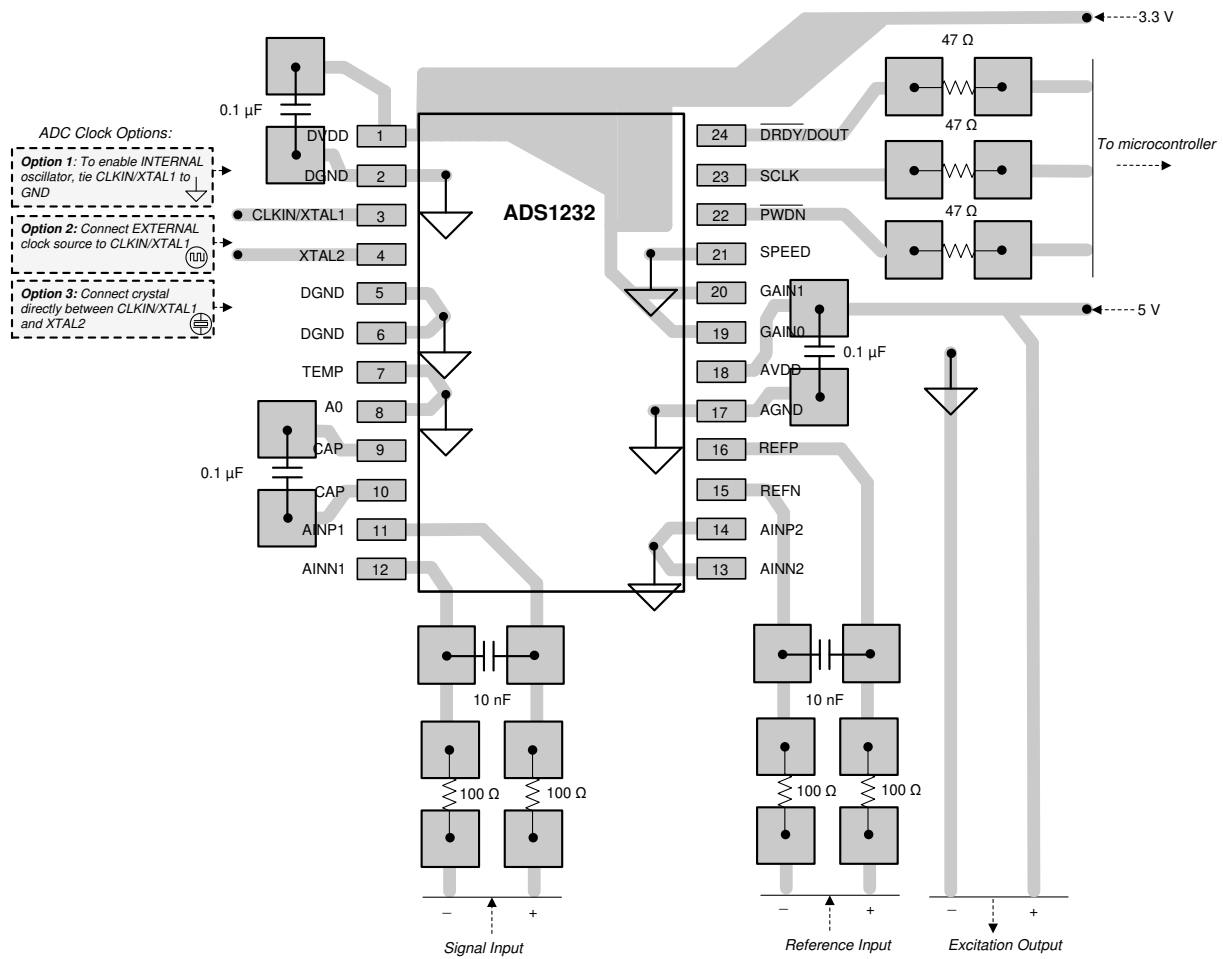
Figure 11-1. ADS1232 Layout Example
