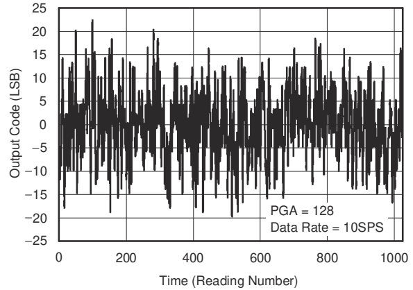
Figure 6-2. Noise Plot
