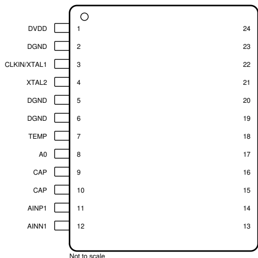
Figure 5-1. ADS1232 PW Package, 24-Pin TSSOP, Top View
