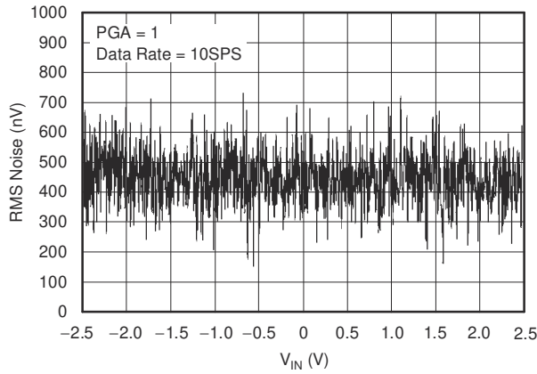
Figure 6-19. Noise vs Input Signal
