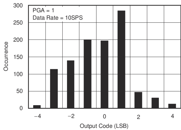
Figure 6-1. Noise Plot
