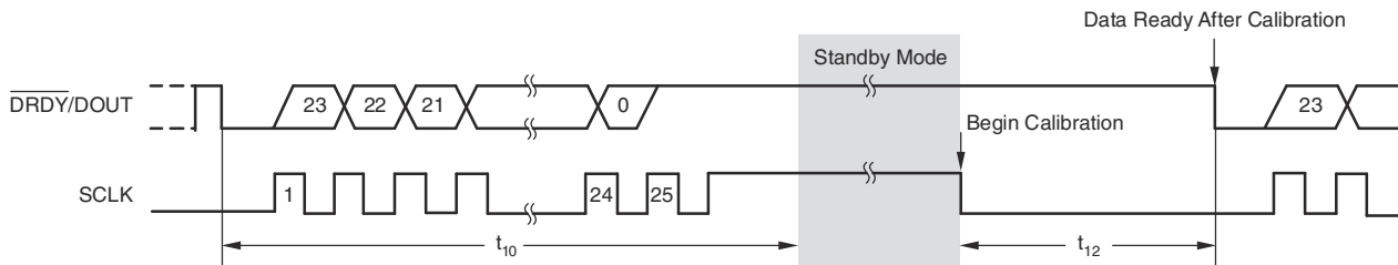
Figure 8-13. Standby Mode With Offset-Calibration Timing (Can be Used for Single Conversions)
