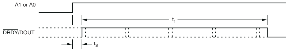
Figure 8-7. Example of Settling Time After Changing the Input Multiplexer
