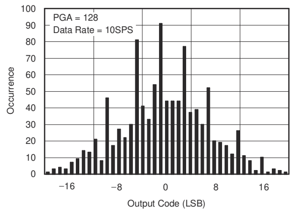
Figure 6-2. Noise Plot
