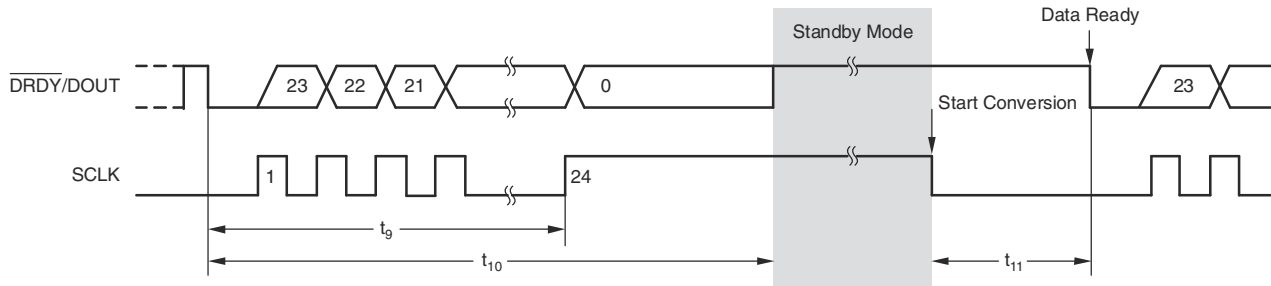
Figure 8-12. Standby Mode Timing (Can be Used for Single Conversions)
