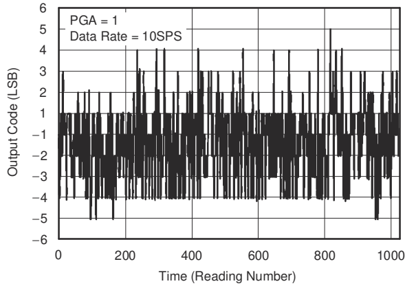
Figure 6-1. Noise Plot
