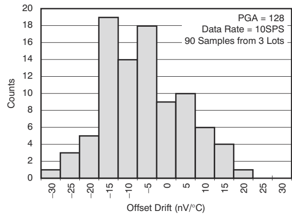
Figure 6-14. Offset Drift (25°C to 105°C)
