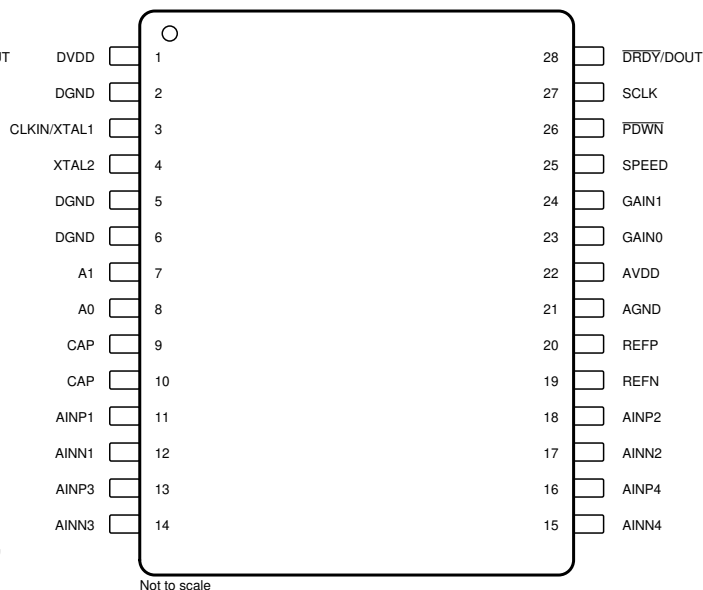
Figure 5-2. ADS1234 PW Package, 28-Pin TSSOP, Top View
