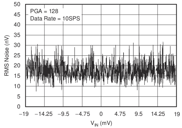
Figure 6-20. Noise vs Input Signal
