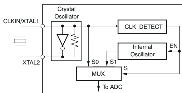
Figure 8-4. Equivalent Circuitry of the Clock Source
