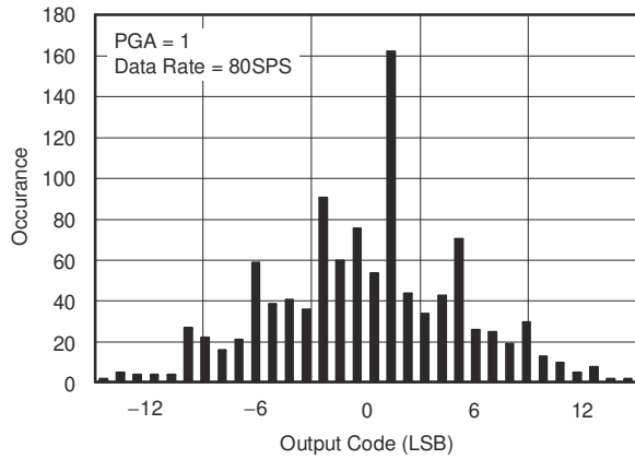
Figure 6-7. Noise Histogram
