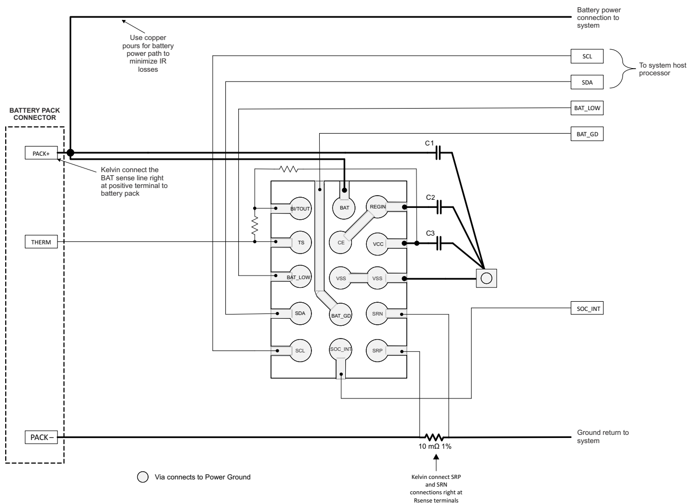
Figure 11-1. Layout Recommendation
