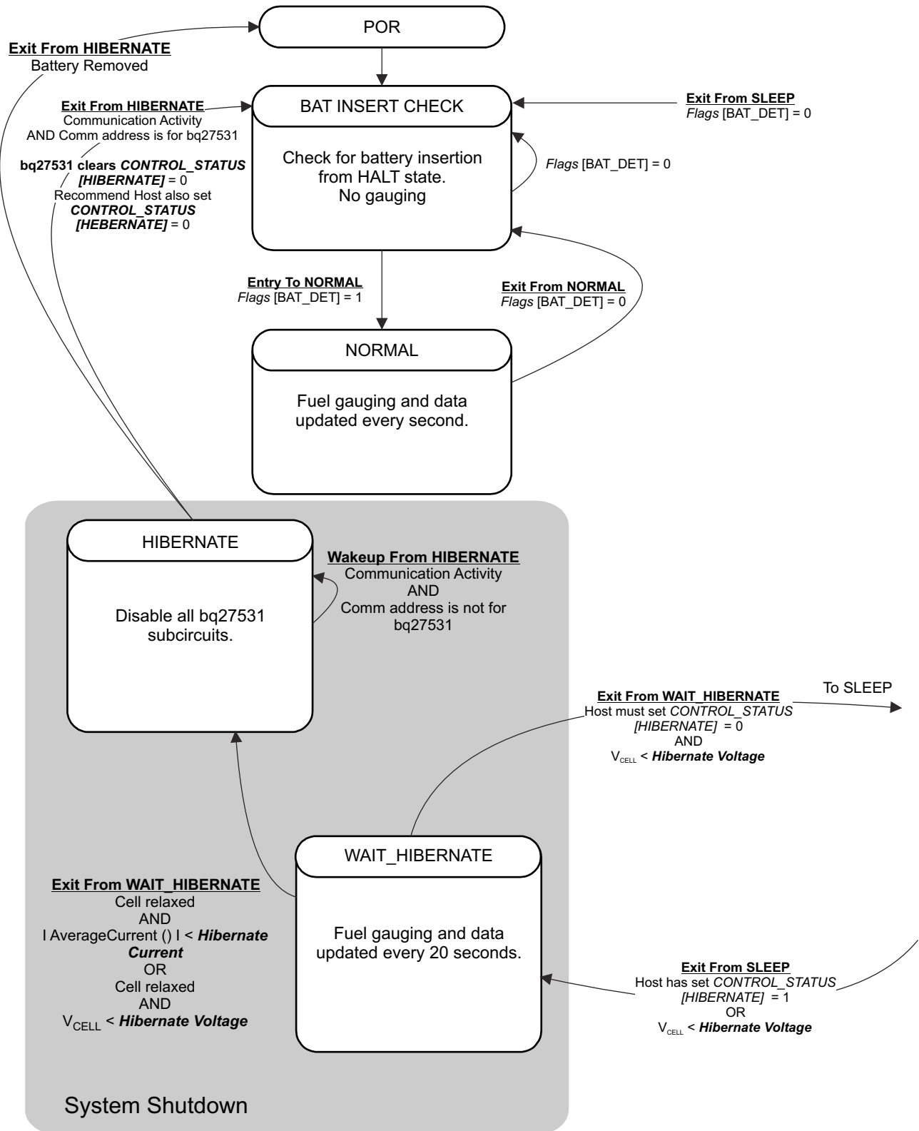
Figure 8-2. Power Mode Diagram—System Shutdown
