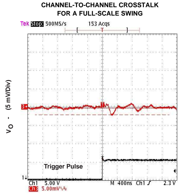
Time - (400 nS/Div)
