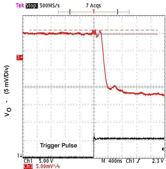
WORST-CASE GLITCH
