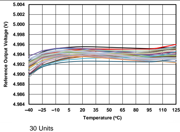
Figure 76. Internal Reference Voltage vs Temperature
