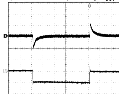
Line Step (LED Mode) (2 x 5 LEDs, 30mA per String, C_{OUT} = 1\mu F )
