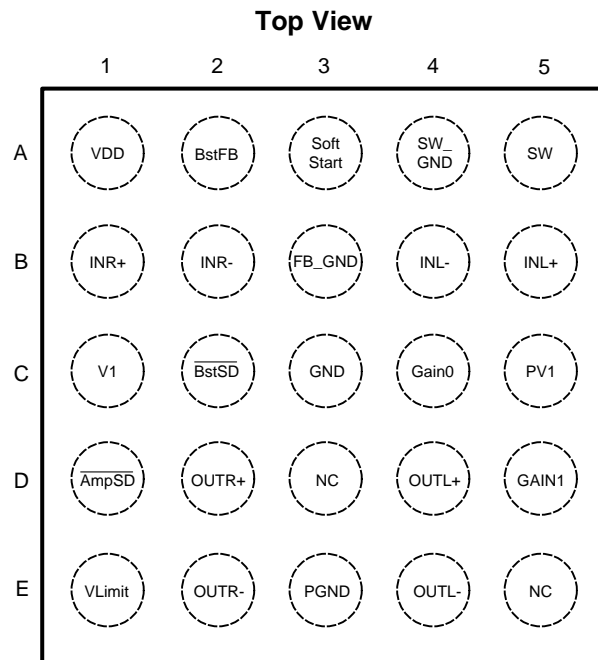
Figure 2. DSBGA Package See Package Number YZR0025AAA
