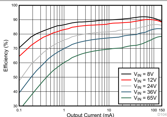
Figure 8-27. Efficiency
