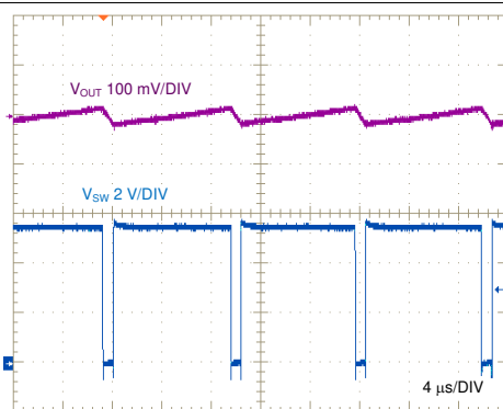
Figure 8-5. SW Node and Output Ripple Voltage, No Load
