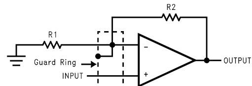
Figure 6-17. Noninverting Amplifier
