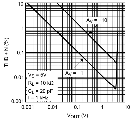
Figure 32. THD+N vs V_{OUT}
