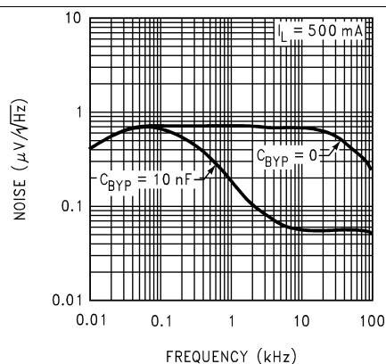
Figure 28. Output Noise Density
