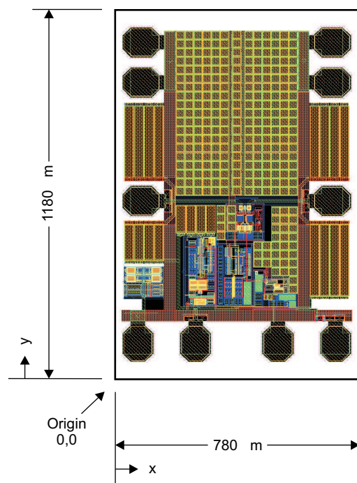
Figure 17. Chip Layout
