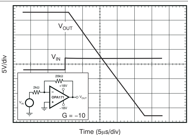
Figure 6-26. Positive Overload Recovery
