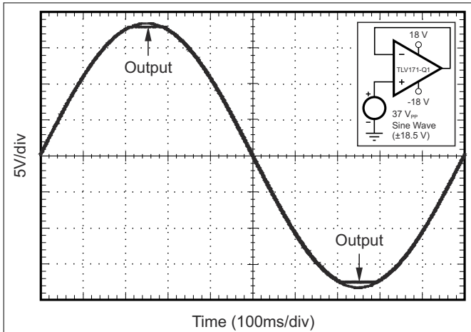
Figure 6-25. No Phase Reversal
