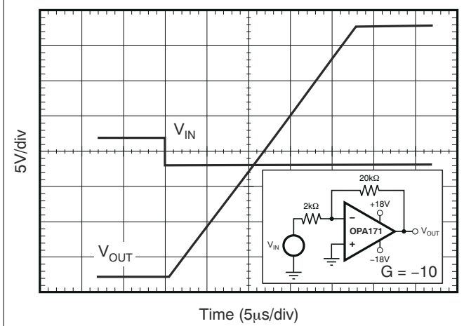
Figure 6-27. Negative Overload Recovery
