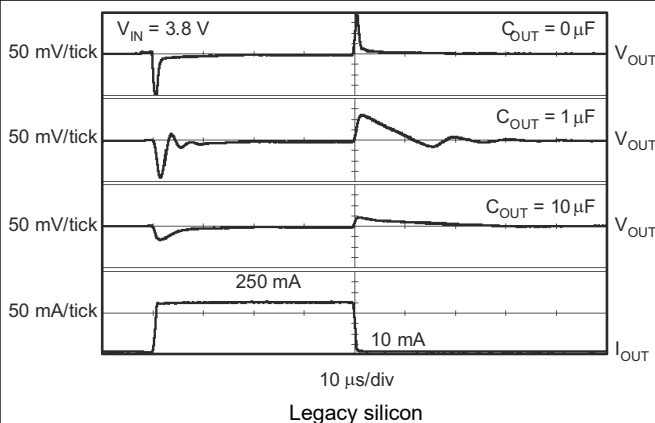
Figure 5-35. TPS73233 Load Transient Response Legacy silicon
