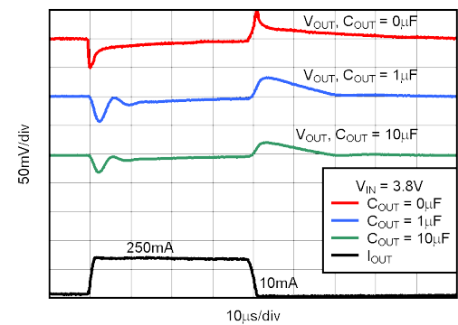
Figure 5-36. TPS73233 Load Transient Response New silicon, M3 suffix
