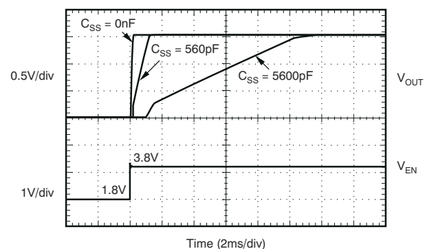
Turn-On Response
