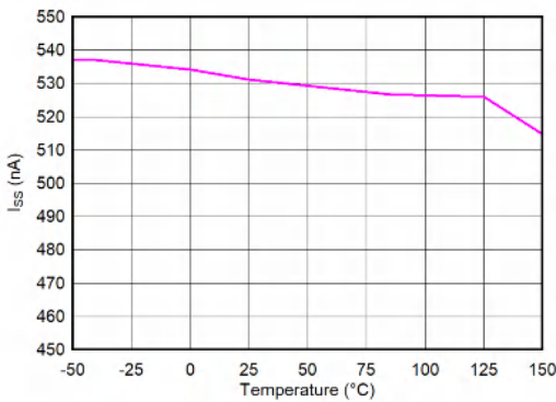
Figure 6-38. Soft-Start Charging Current (I SS ) vs Temperature (T J )
