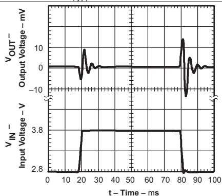
I_{OUT} = 100\text{ mA} , C_{OUT} = 1\text{ }\mu\text{F} , C_{BYPASS} = 0.01\text{ }\mu\text{F}
