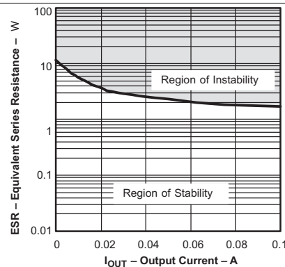
V_{IN} = 5.5\text{ V} , C_{OUT} = 1\text{ }\mu\text{F} , T_J = -40^\circ\text{C} to 125^\circ\text{C}
