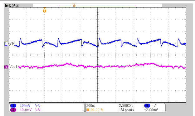
Figure 9-25. Output and Input Voltage Ripple
