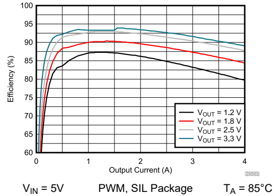
Figure 9-9. Efficiency versus Output Current
