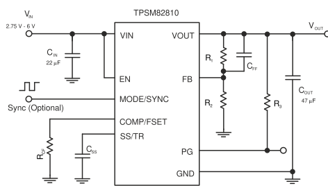
Schematic
