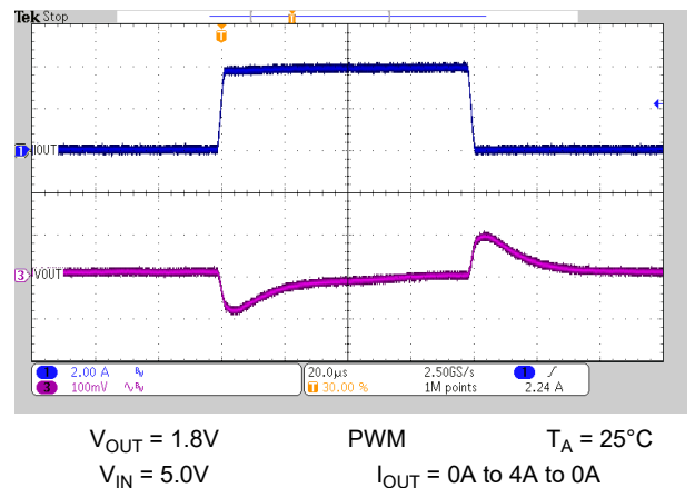
Figure 9-23. Load Transient Response
