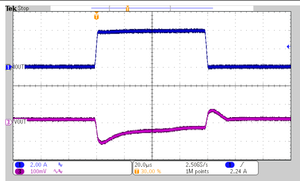
Figure 9-24. Load Transient Response
