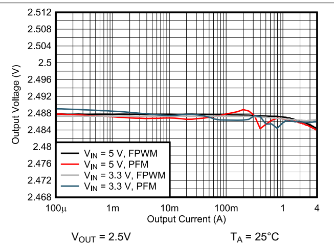
Figure 9-19. Output Voltage versus Output Current
