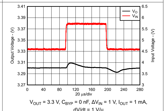
Figure 7-8. Line Transient Response for New Chip
