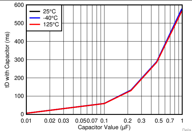
Figure 40. Reset Time Delay vs Small Capacitor Values (Data Taken with TPS3840PL16)
