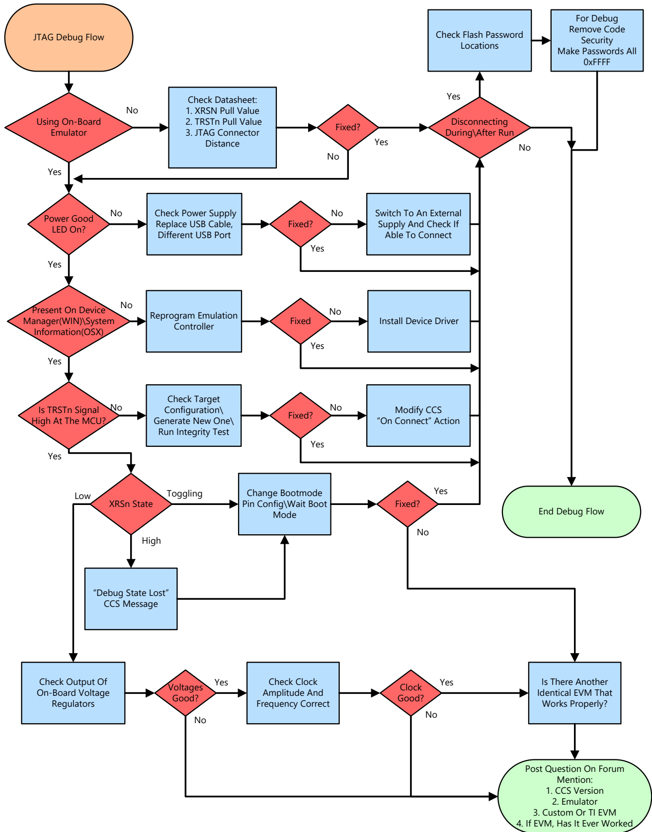
Figure 3. JTAG Debug Flow
