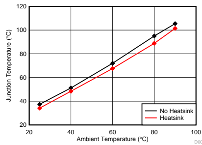
Figure 3. Dyrystone(Core 1) @ OPP_NOM (Junction Temp vs Ambient Temp)
