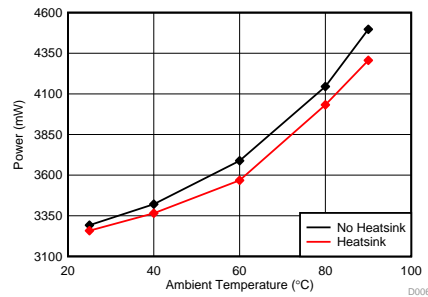
Figure 6. Dyrystone(Core 1) @ OPP_OD (Power Consumption vs Ambient Temp)
