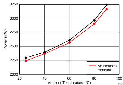
Figure 2. OS Idle - OPP_NOM (Power Consumption vs Ambient Temp)
