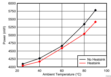
Figure 8. Dyrystone(Core 1) @ OPP_HIGH (Power Consumption vs Ambient Temp)
