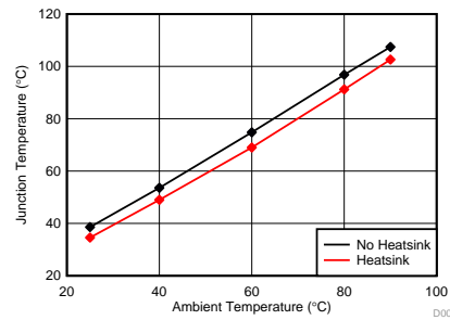
Figure 5. Dyrystone(Core 1) @ OPP_OD (Junction Temp vs Ambient Temp)
