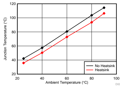
Figure 7. Dyrystone(Core 1) @ OPP_HIGH (Junction Temp vs Ambient Temp)
