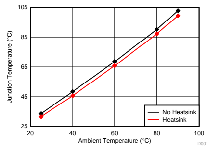
Figure 1. OS Idle - OPP_NOM (Junction Temp vs Ambient Temp)
