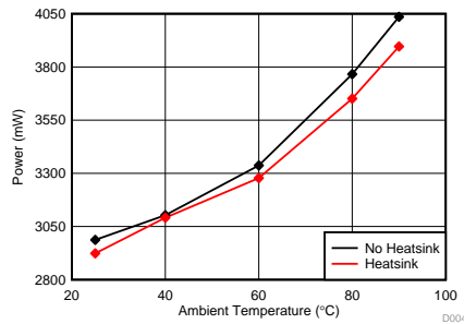
Figure 4. Dyrystone(Core 1) @ OPP_NOM (Power Consumption vs Ambient Temp)
