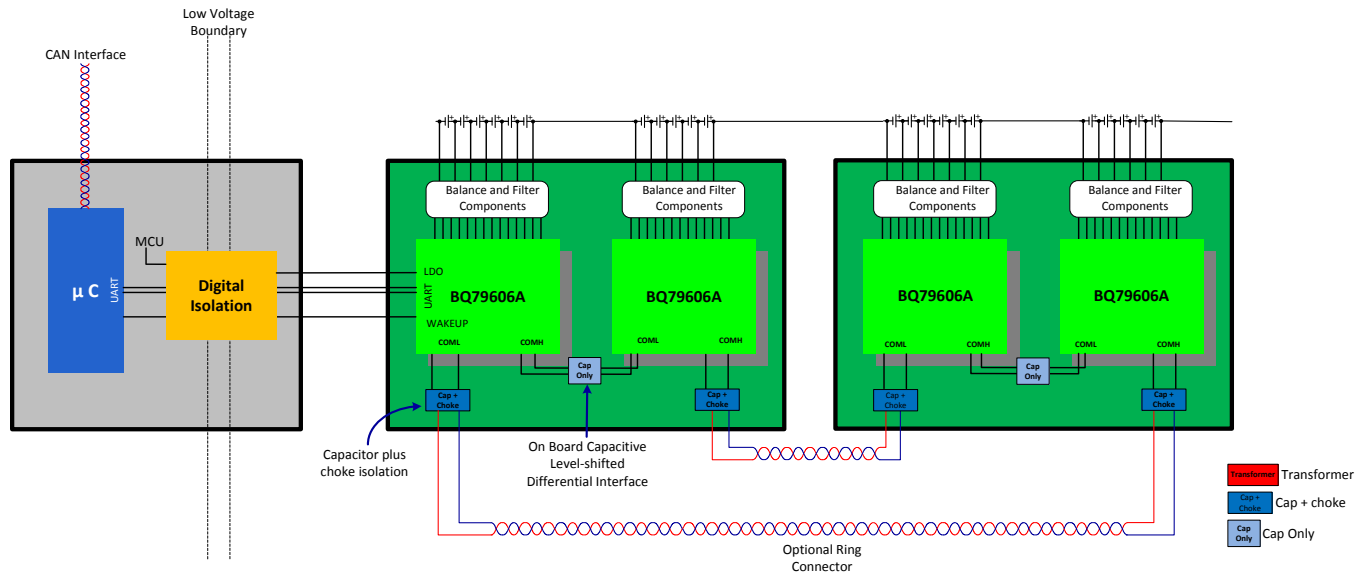
FIG 66. System Application with Integrated Base Device
