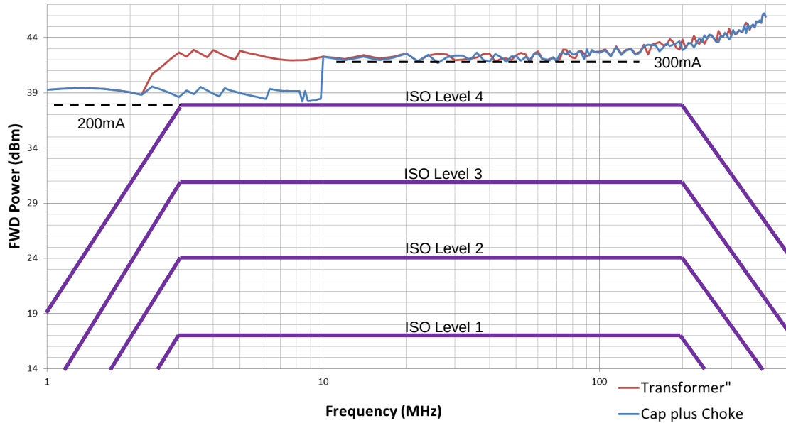
FIG 62. BCI of Transformer Isolation vs. Capacitive Plus Choke Isolation, 1.7m Cable
