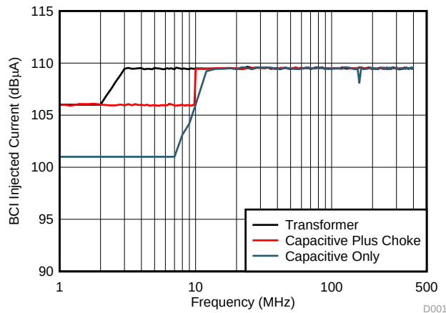
FIG 1. BCI Performance For capacitive Isolation, Capacitive Plus Choke, and Transformer Isolation
