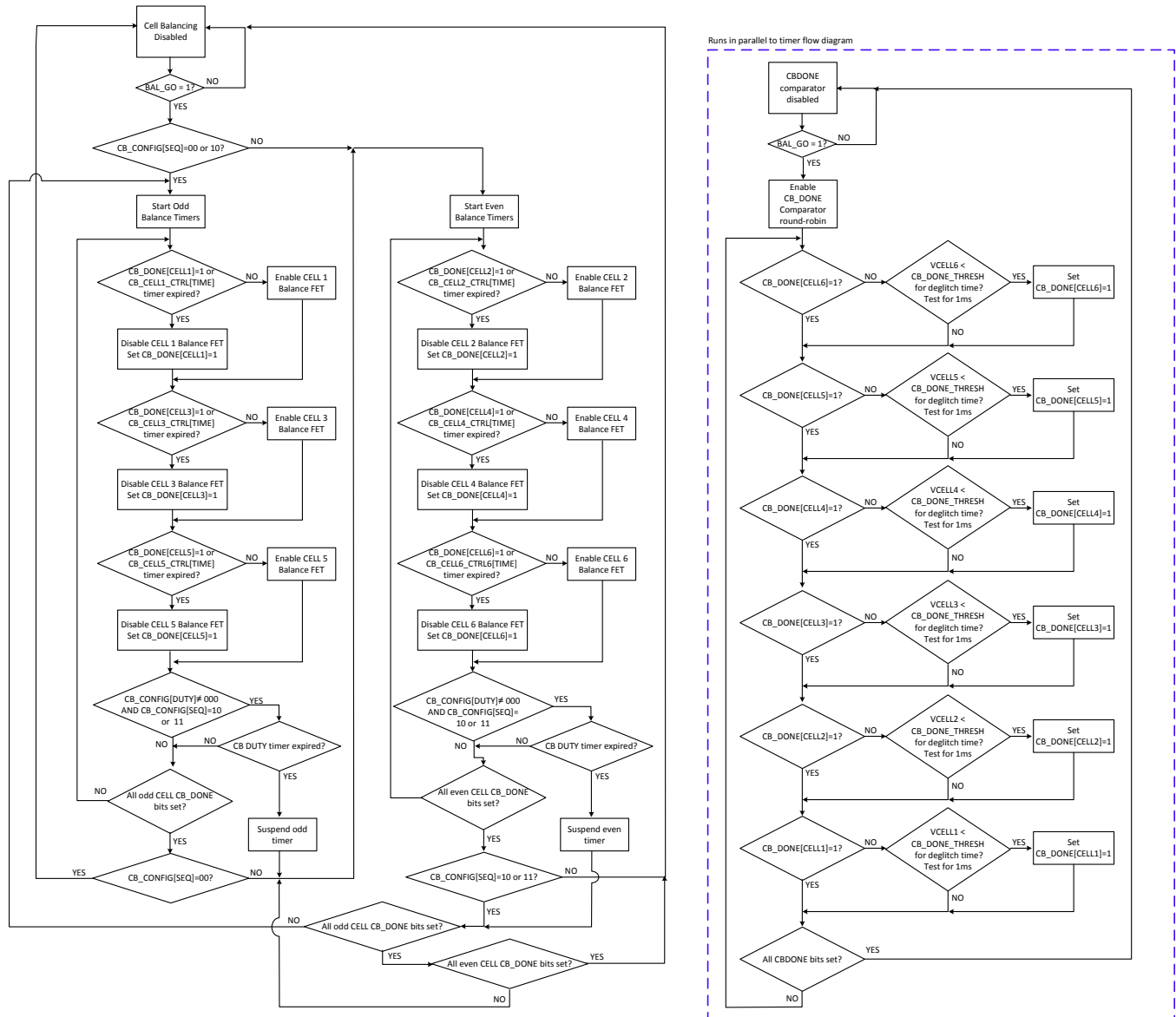
19. Flow Diagram for Cell Balancing
