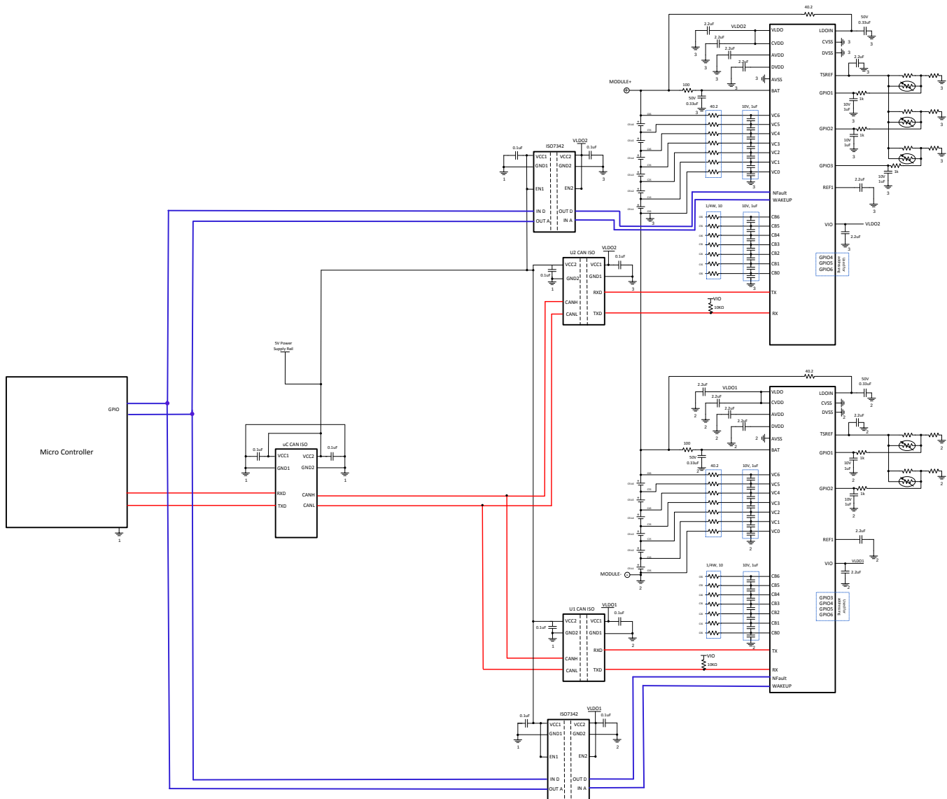
63. Typical Module Application Circuit with Multi-Drop Configuration
