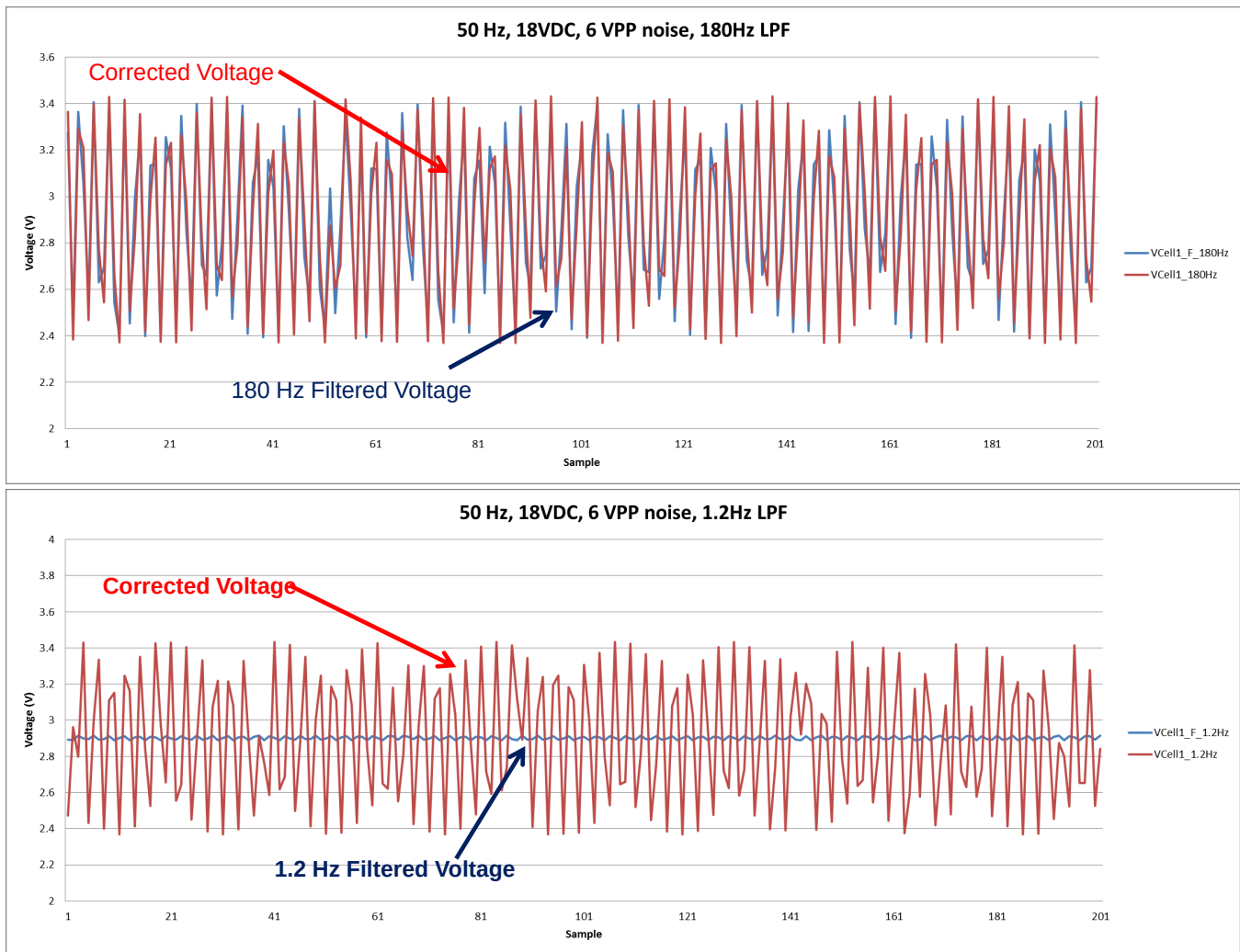
FIG 60. Digital Low Pass Filter Results
