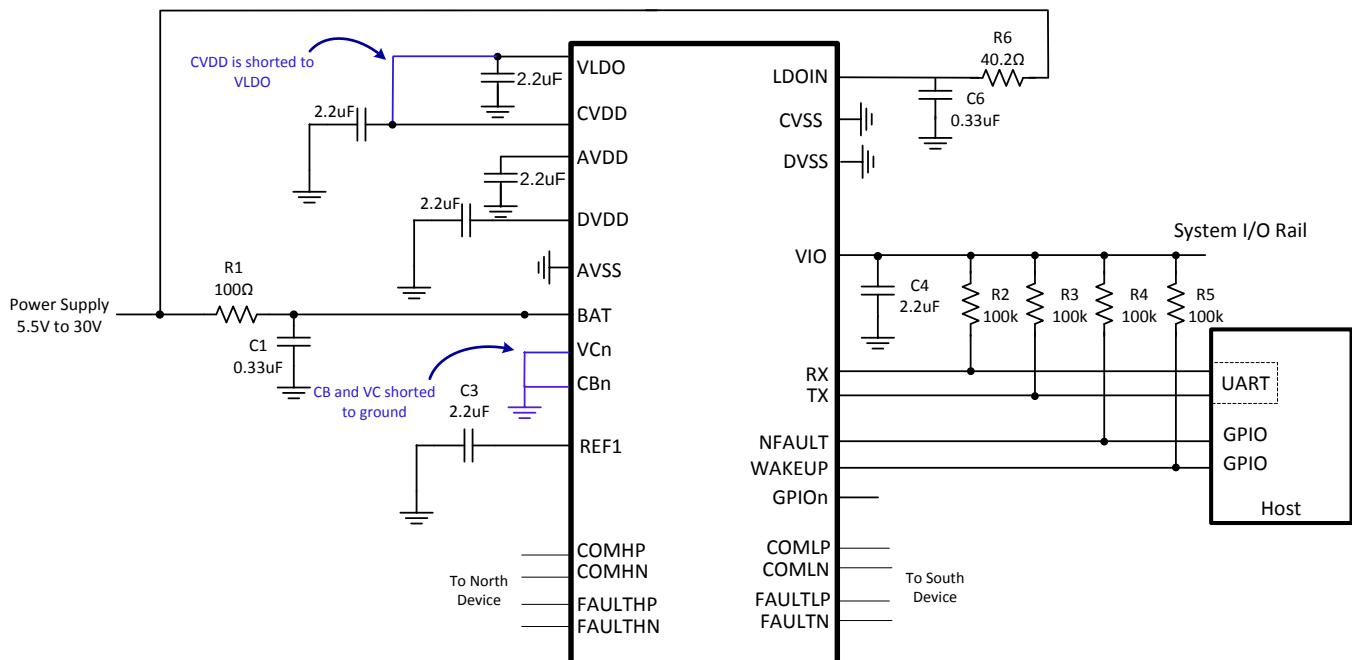
✎ 56. Typical Application Circuit for Bridge Device for Input Supply From 5.5V to 30V
