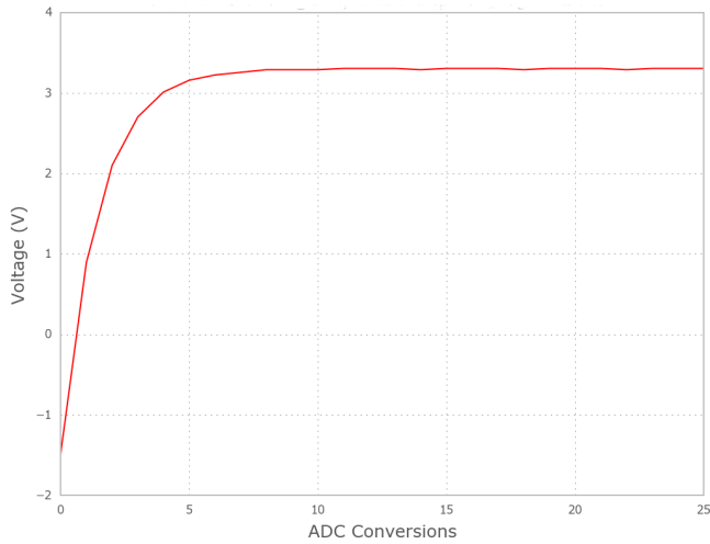
Reported Voltage w/3.3 V Input at f_C = 180.1 Hz FIG 8. FILSHIFT = 3'b000 Step Response, DR=256
