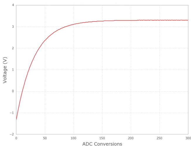
Reported Voltage w/3.3 V Input at f_C = 9.8 Hz FIG 12. FILSHIFT = 3'b100 Step Response, DR=256
