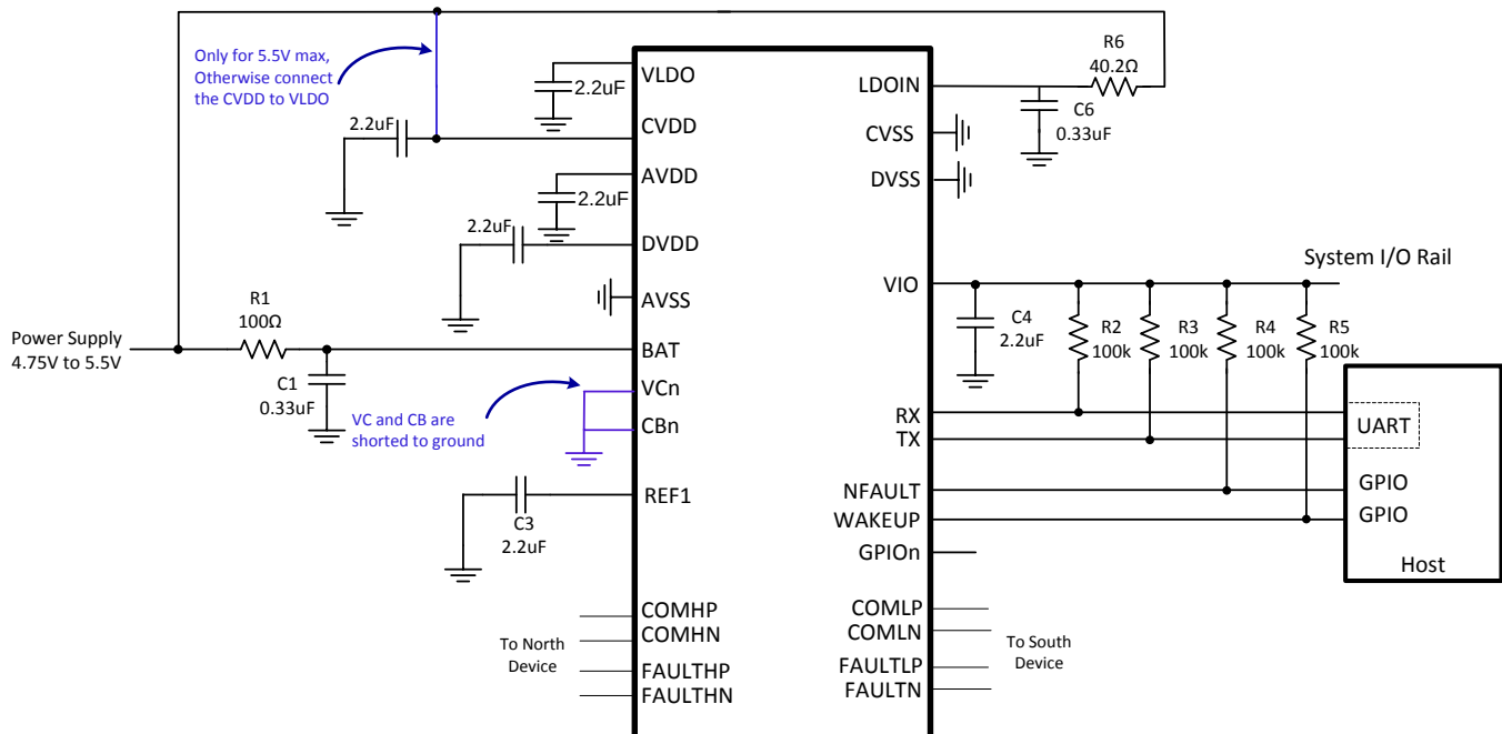
✎ 55. Typical Application Circuit for Bridge Device for Input Supply From 4.75V to 5.5V
