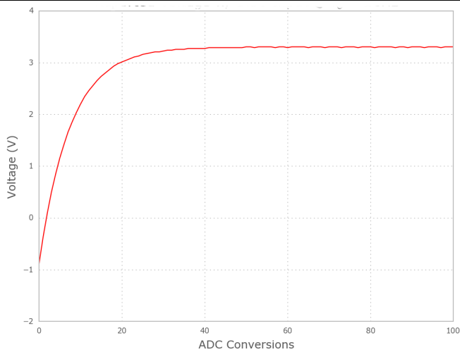
Reported Voltage w/3.3 V Input at f_C = 40.1 Hz FIG 10. FILSHIFT = 3'b010 Step Response, DR=256
