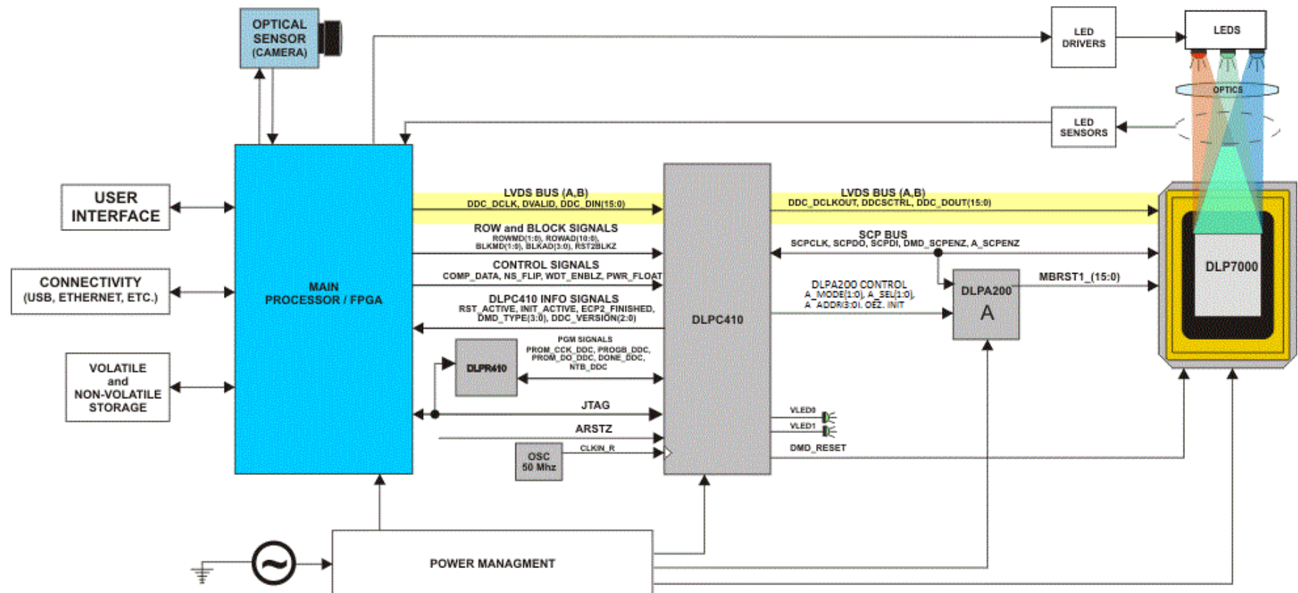
9-1. DLPC410 and DLP7000 Embedded Example Block Diagram
