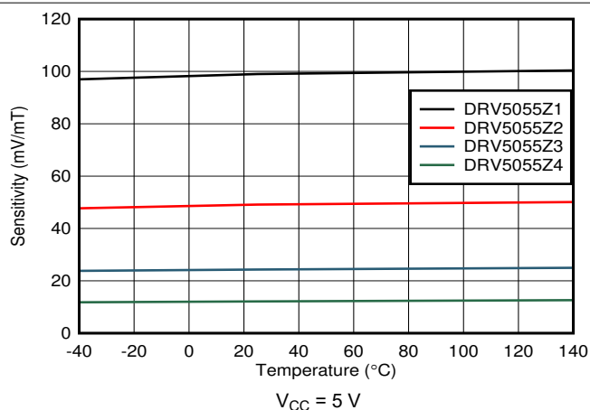
图 5-8. Sensitivity vs Temperature
