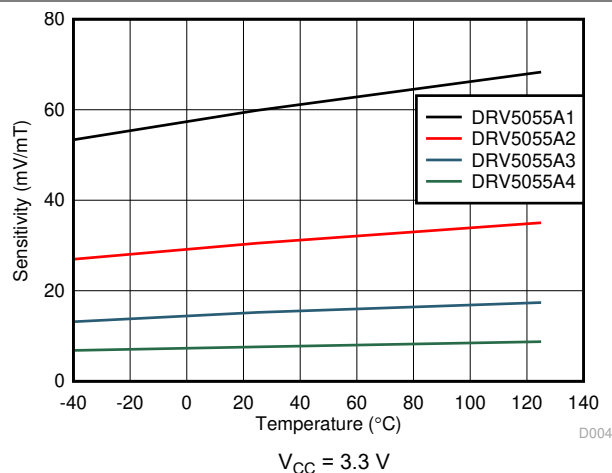
图 5-5. Sensitivity vs Temperature
