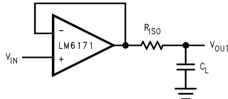
Figure 7-5. Isolation Resistor Used to Drive Capacitive Load
