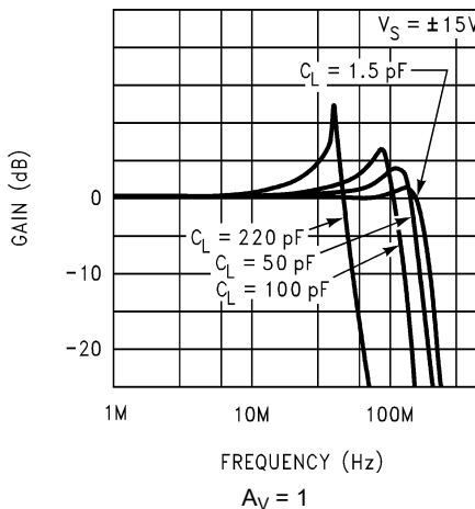
図 5-94. Closed-Loop Frequency Response vs Capacitive Load
