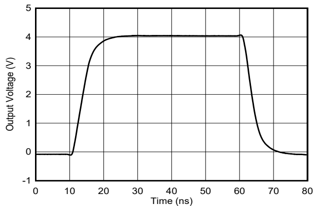
图 5-27. Large-Signal Pulse Response
