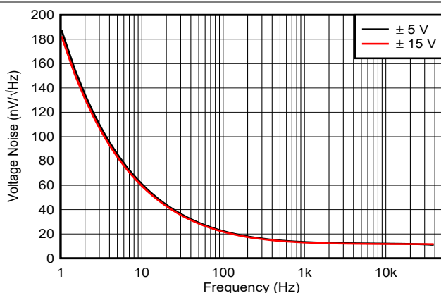
図 5-19. Input Voltage Noise vs Frequency
