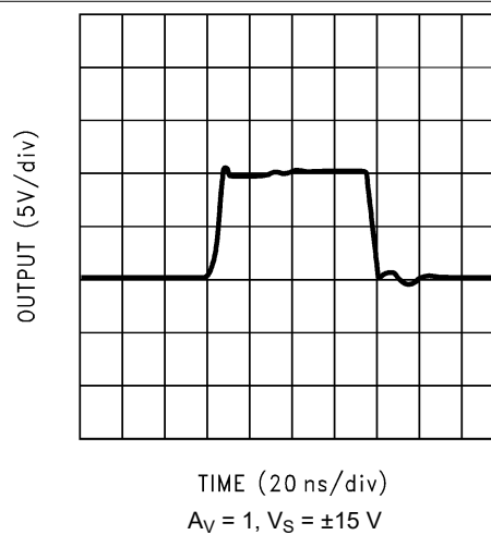
5-82. Large-Signal Pulse Response
