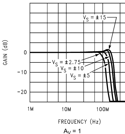
図 5-92. Closed-Loop Frequency Response vs Supply Voltage
