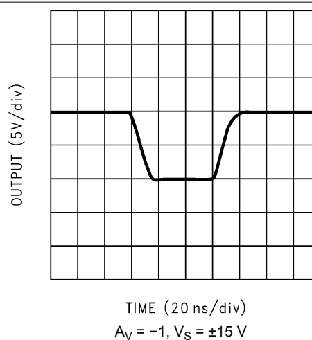
5-80. Large-Signal Pulse Response
