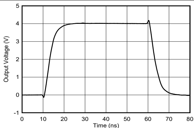
図 5-31. Large-Signal Pulse Response
