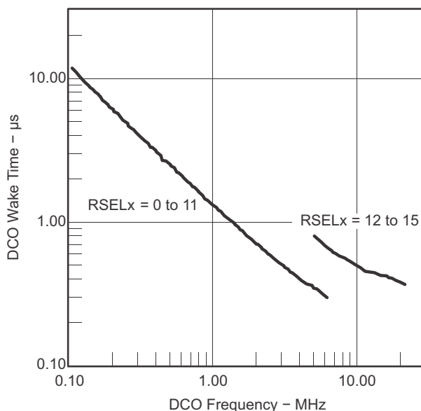
Figure 18. DCO Wake-Up Time From LPM3 vs DCO Frequency
