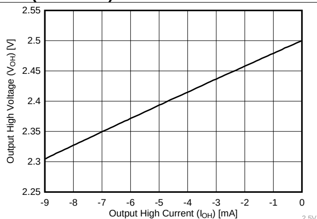
Fig. 8. Typical Output High Voltage of 2.5 V (25°C)
