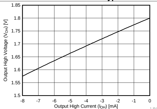
Fig. 7. Typical Output High Voltage of 1.8 V (25°C)
