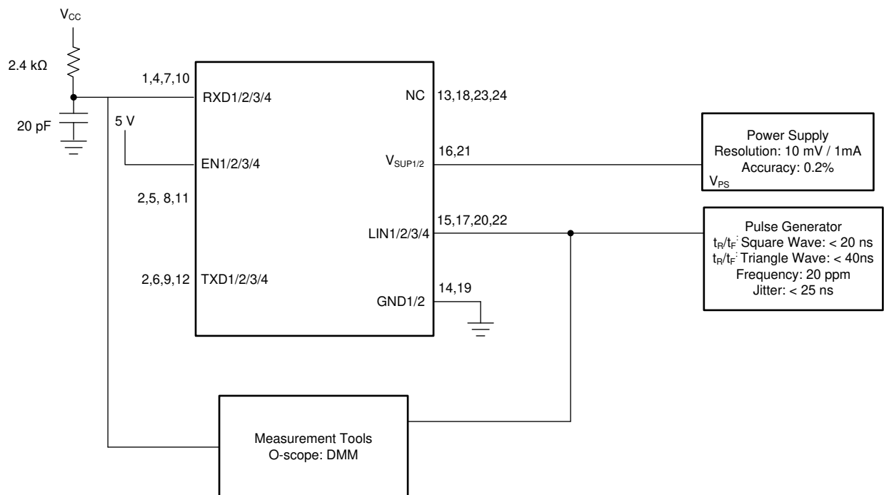
7-13. Propagation Delay Test Circuit
