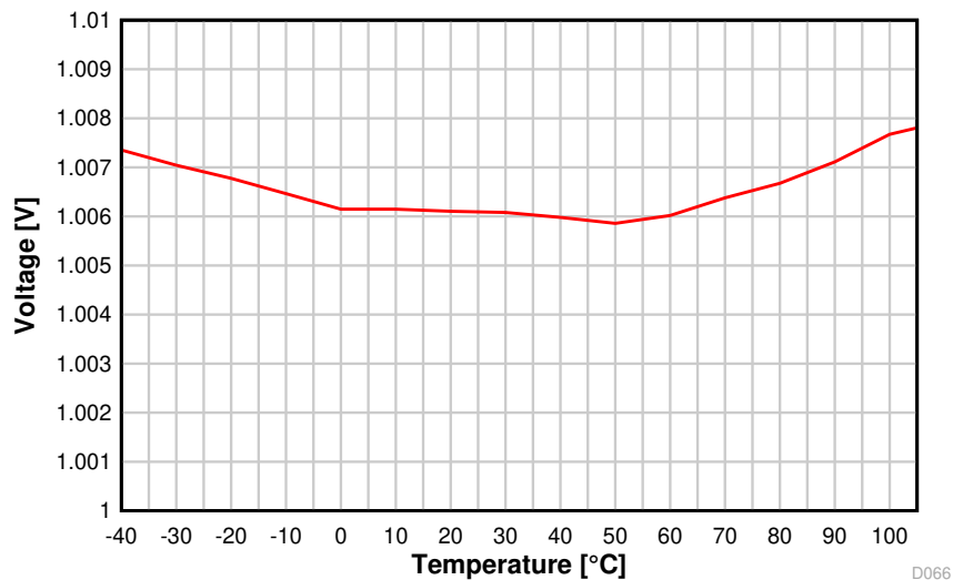
8-37. ADC Accuracy vs. Temperature
