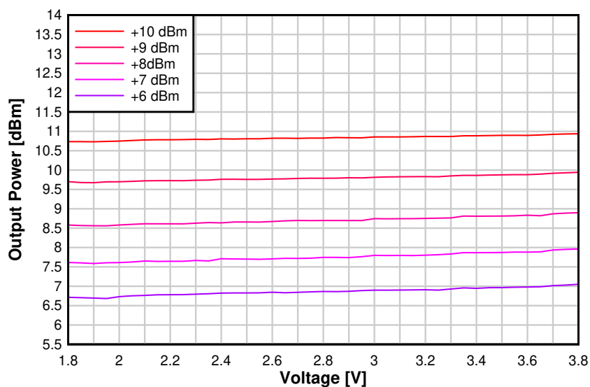
8-28. Output Power vs. Supply Voltage (VDD5) (2.44 GHz, +10 dBm PA)
