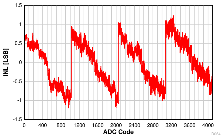
8-35. INL vs. ADC Code
