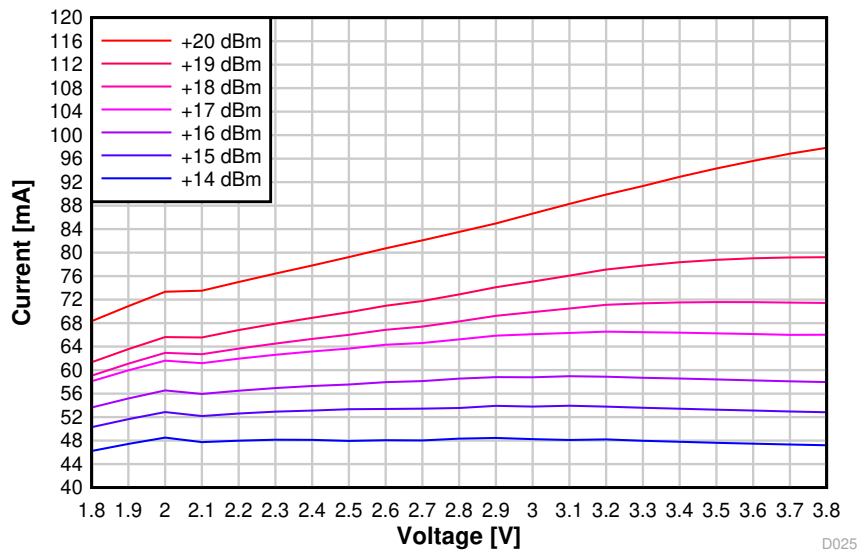
8-12. TX Current vs. Supply Voltage (VDD5) (BLE 1 Mbps, 2.44 GHz, +20 dBm PA)
