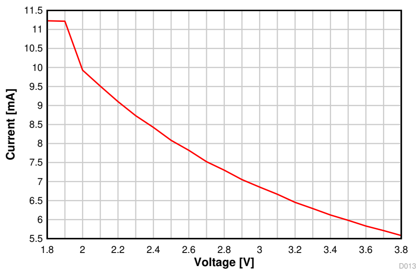
8-7. RX Current vs. Supply Voltage (VDD5) (BLE 1 Mbps, 2.44 GHz)
