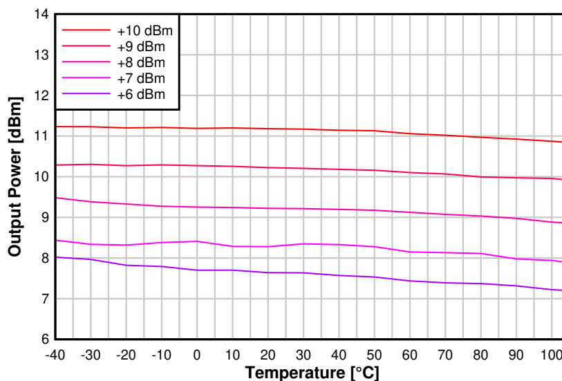
8-24. Output Power vs. Temperature (2.44 GHz, +10 dBm PA)
