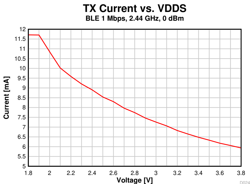
8-11. TX Current vs. Supply Voltage (VDD5) (BLE 1 Mbps, 2.44 GHz)
