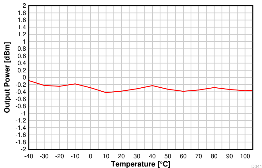
8-21. Output Power vs. Temperature (BLE 1 Mbps, 2.44 GHz)
