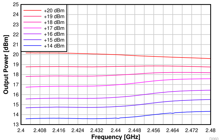
8-31. Output Power vs. Frequency (BLE 1 Mbps, 2.44 GHz, +20 dBm PA)
