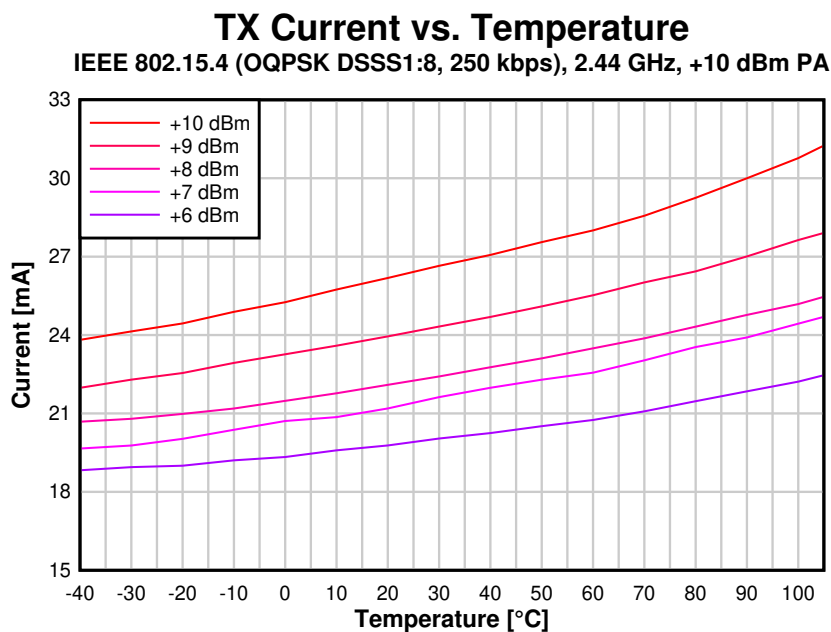
8-10. TX Current vs. Temperature (250 kbps, 2.44 GHz, +10 dBm PA)
