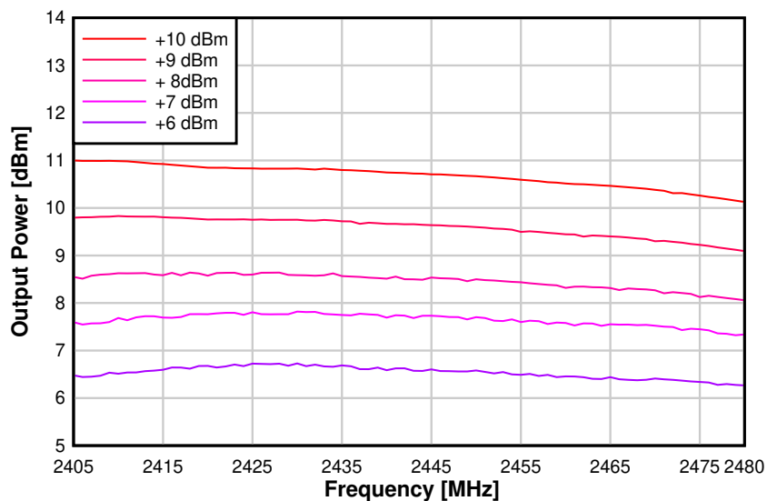
8-32. Output Power vs. Frequency (250 kbps, +10 dBm PA)
