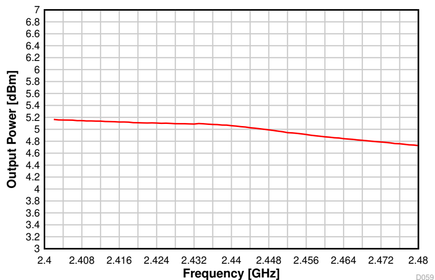
8-30. Output Power vs. Frequency (BLE 1 Mbps, 2.44 GHz, +5 dBm)
