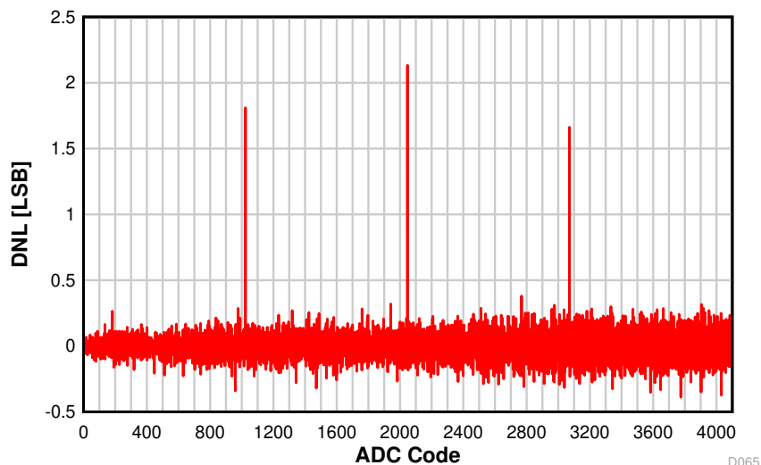
8-36. DNL vs. ADC Code
