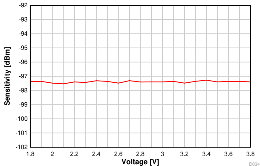
8-18. Sensitivity vs. Supply Voltage (VDDS) (BLE 1 Mbps, 2.44 GHz)
