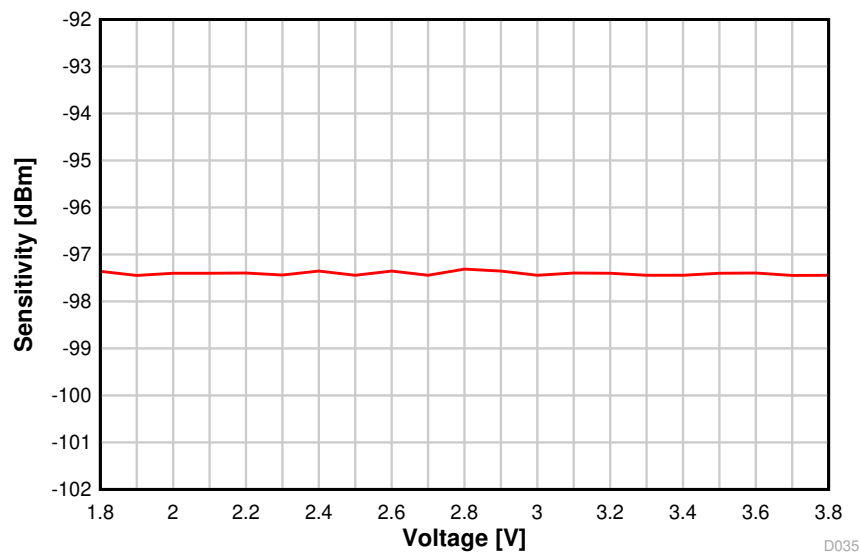
8-19. Sensitivity vs. Supply Voltage (VDDS) (BLE 1 Mbps, 2.44 GHz, DCDC Off)
