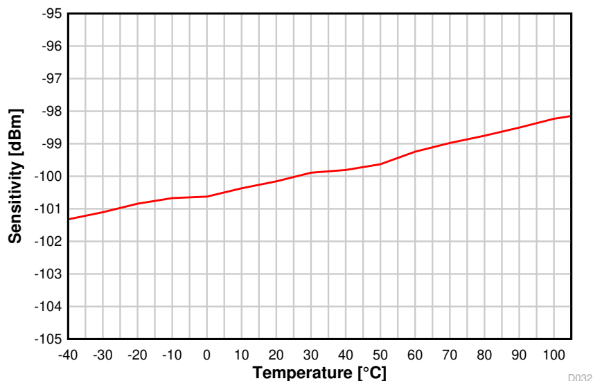
8-17. Sensitivity vs. Temperature (250 kbps, 2.44 GHz)
