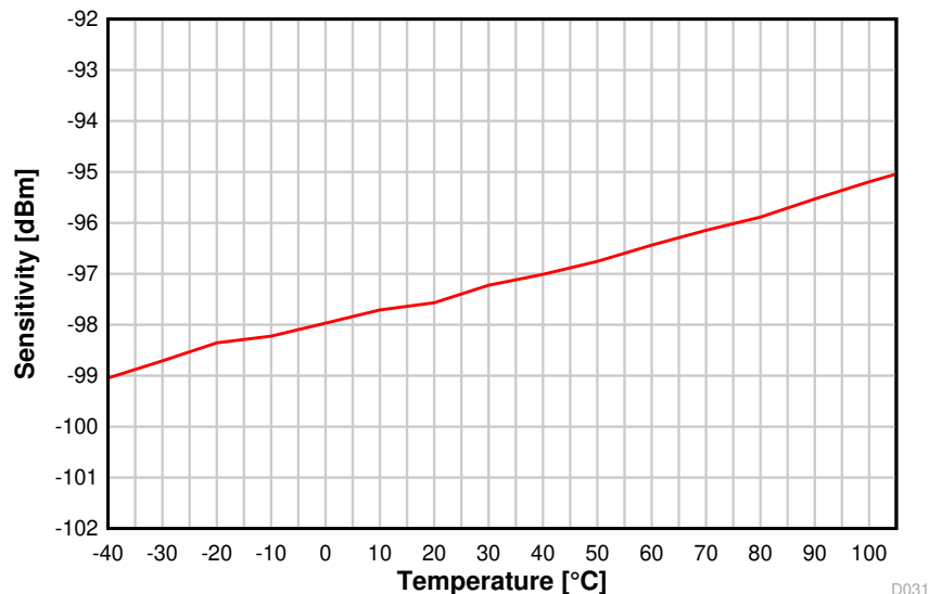
8-16. Sensitivity vs. Temperature (BLE 1 Mbps, 2.44 GHz)
