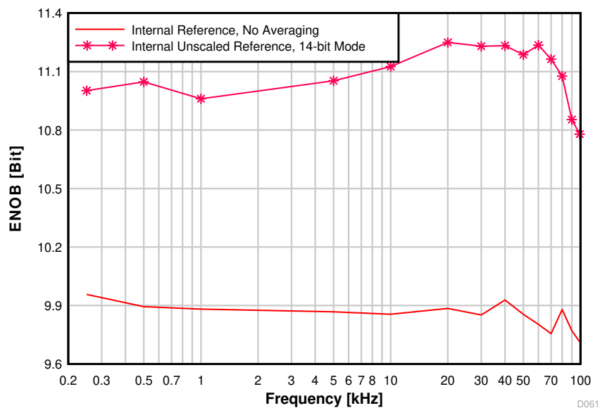
8-33. ENOB vs. Input Frequency
