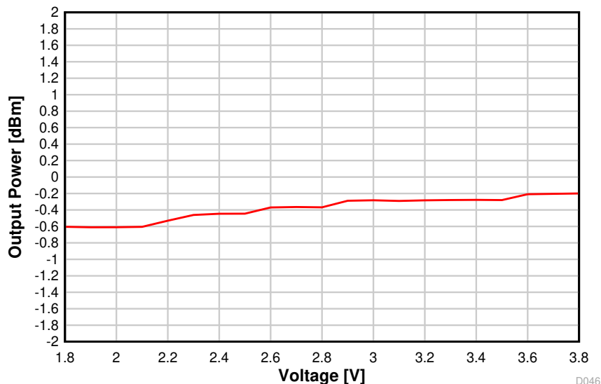
8-25. Output Power vs. Supply Voltage (VDDS) (BLE 1 Mbps, 2.44 GHz)
