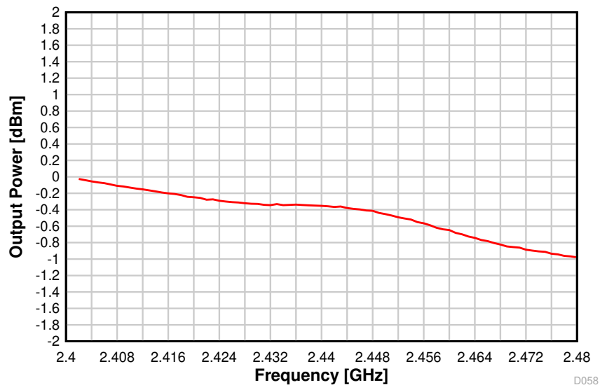
8-29. Output Power vs. Frequency (BLE 1 Mbps, 2.44 GHz)
