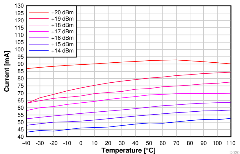
Figure 8-9. TX Current vs. Temperature (BLE 1 Mbps, 2.44 GHz, VDD = 3.3 V)
