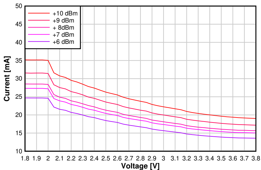
8-13. TX Current vs. Supply Voltage (VDD5) (250 kbps, 2.44 GHz, +10 dBm PA)
