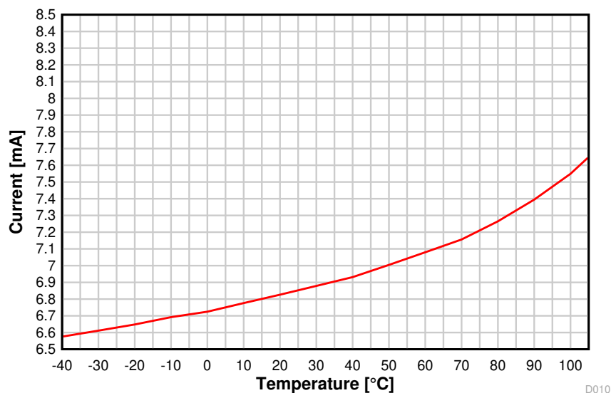
8-6. RX Current vs. Temperature (BLE 1 Mbps, 2.44 GHz)
