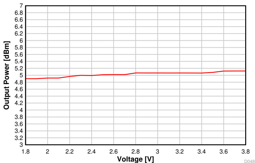
8-26. Output Power vs. Supply Voltage (VDDS) (BLE 1 Mbps, 2.44 GHz, +5 dBm)
