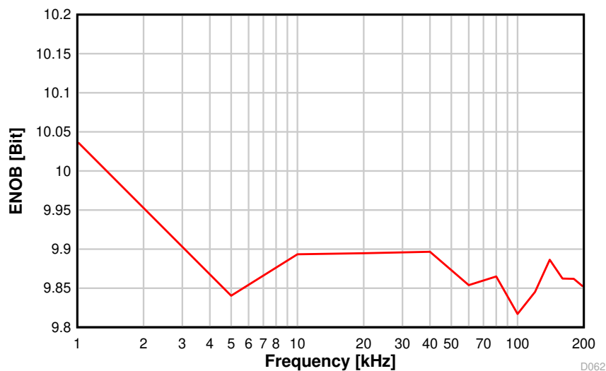
8-34. ENOB vs. Sampling Frequency
