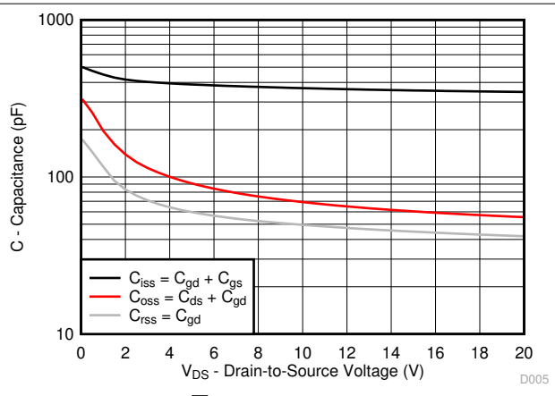
Figure 4-5. Capacitance
