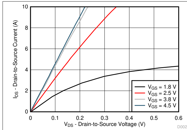
Figure 4-2. Saturation Characteristics
