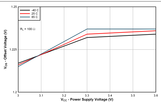
FIG 6. Offset Voltage vs Power Supply Voltage
