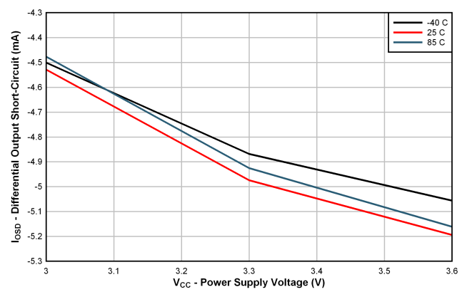
FIG 4. Differential Output Short-Circuit Current vs Power Supply Voltage
