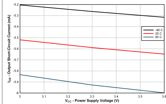
FIG 3. Output Short-Circuit Current vs Power Supply Voltage
