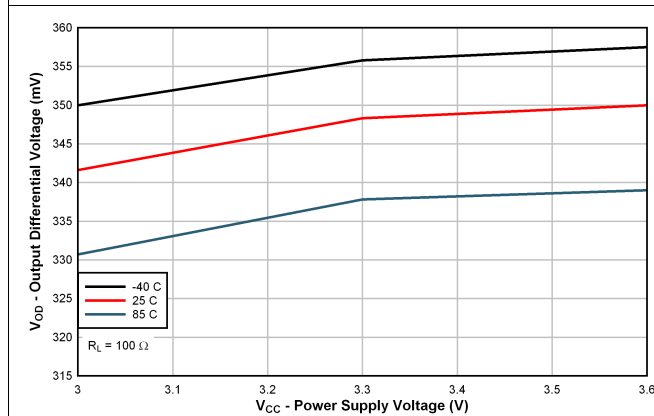
FIG 5. Output Differential Voltage vs Power Supply Voltage
