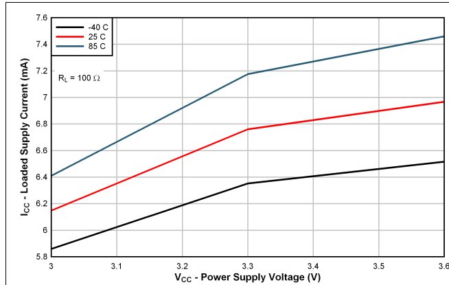
FIG 1. Loaded Supply Current vs Power Supply Voltage
