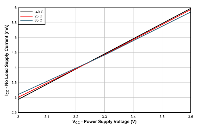
FIG 2. No Load Supply Current vs Power Supply Voltage
