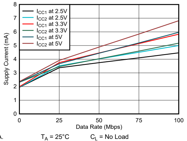
6-8. ISO7731 Supply Current vs Data Rate (With No Load)
