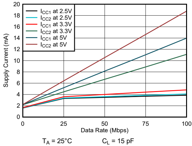
6-5. ISO7730 Supply Current vs Data Rate (With 15-pF Load)
