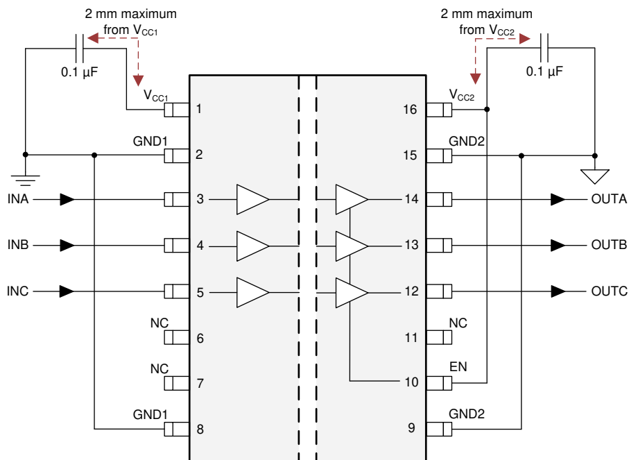
図 9-2. Typical ISO7730 Circuit Hook-Up
