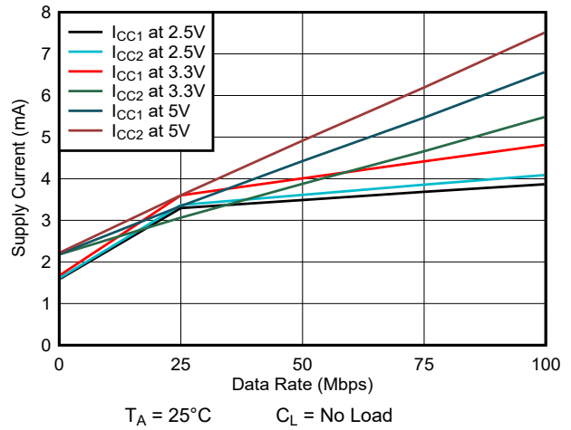
6-6. ISO7730 Supply Current vs Data Rate (With No Load)
