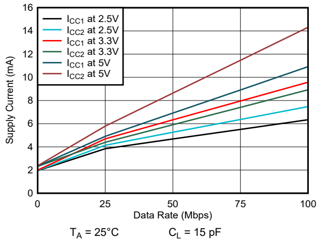
6-7. ISO7731 Supply Current vs Data Rate (With 15-pF Load)
