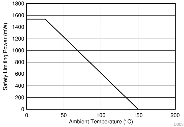
6-3. Thermal Derating Curve for Safety Limiting Power per VDE for DW-16 Package
