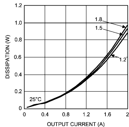
Dissipation 5V Input @ 25^\circ\text{C}
