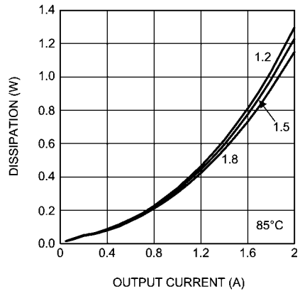
Dissipation 5V Input @ 85°C
