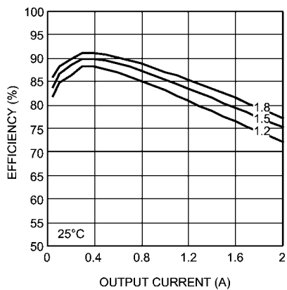
Efficiency 5V Input @ 25^\circ\text{C}
