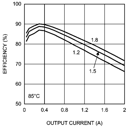
Efficiency 5V Input @ 85°C
