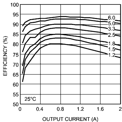
Efficiency 12V Input @ 25°C
