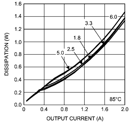
Dissipation 20V Input @ 85°C
