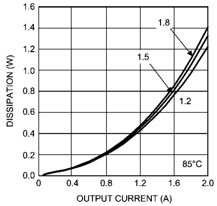
Dissipation 4.5V Input @ 85°C
