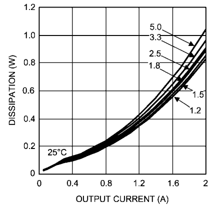
Dissipation 8V Input @ 25°C
