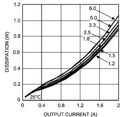
Dissipation 12V Input @ 25°C
