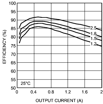
Efficiency 8V Input @ 25°C
