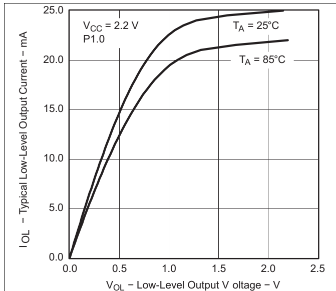
Figure 5-5. Typical Low-Level Output Current vs Low-Level Output Voltage
