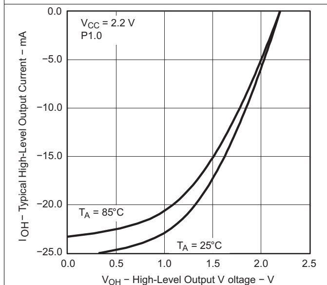
Figure 5-7. Typical High-Level Output Current vs High-Level Output Voltage
