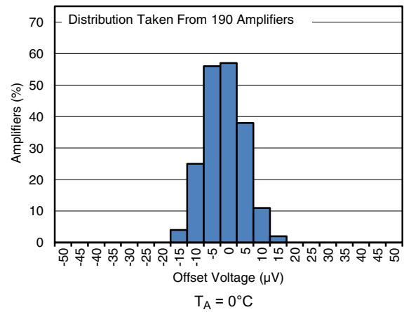
6-4. Offset Voltage Production Distribution at 0°C
