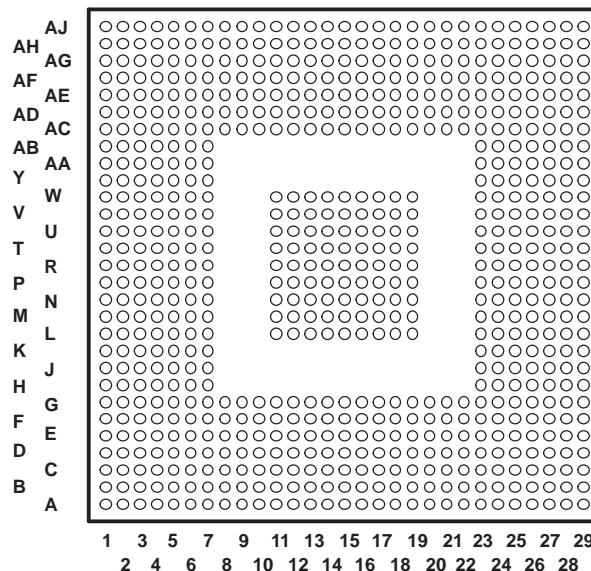
TZ/GTZ 697-PIN BALL GRID ARRAY (BGA) PACKAGE (BOTTOM VIEW)
