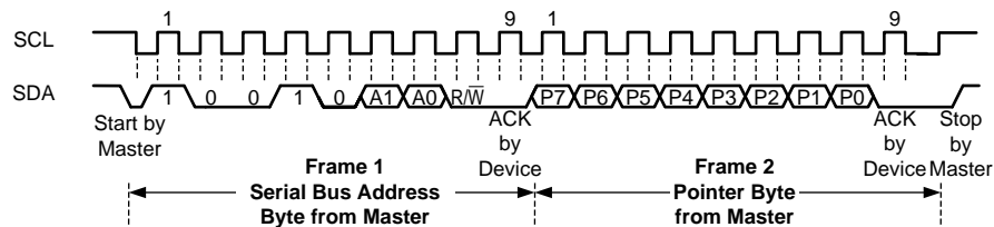
15. Two-Wire Timing Diagram for Write Pointer Byte
