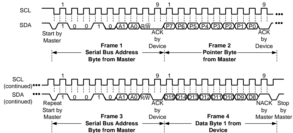
17. Two-Wire Timing Diagram for Pointer Set Followed by a Repeat Start and Single-Byte Read Format
