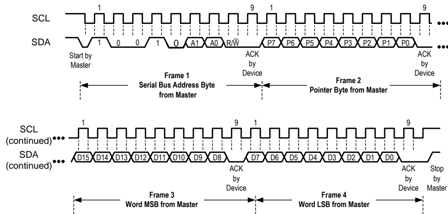
16. Two-Wire Timing Diagram for Write Pointer Byte and Value Word
