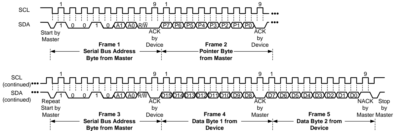
18. Two-Wire Timing Diagram for Pointer Byte Set Followed by a Repeat Start and Word (Two-Byte) Read
