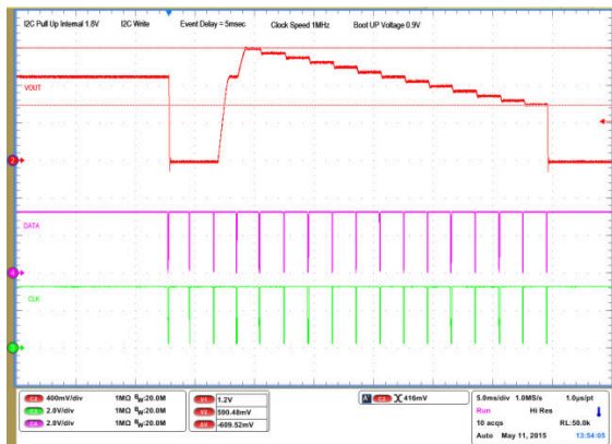
Figure 5-15. 6 Sequenced Events – I2C Write/Read
