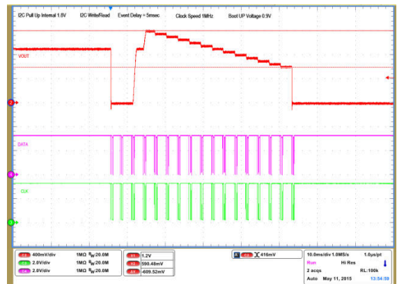
Figure 5-16. 6 Sequenced Events – I2C Write/Read with PEC
