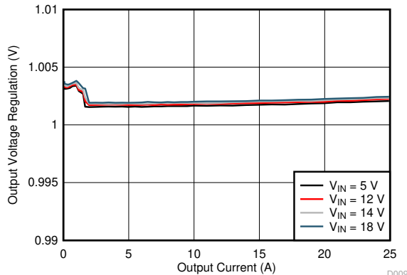
8-3. Output Voltage Regulation vs. Output Current
