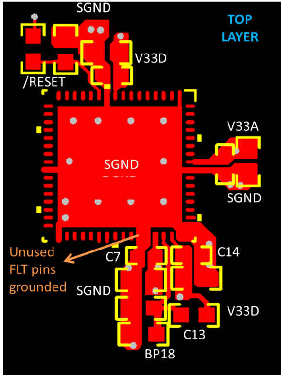
12-14. UCD3138 and UCD3138064 64 Pin Layout Top Layer
