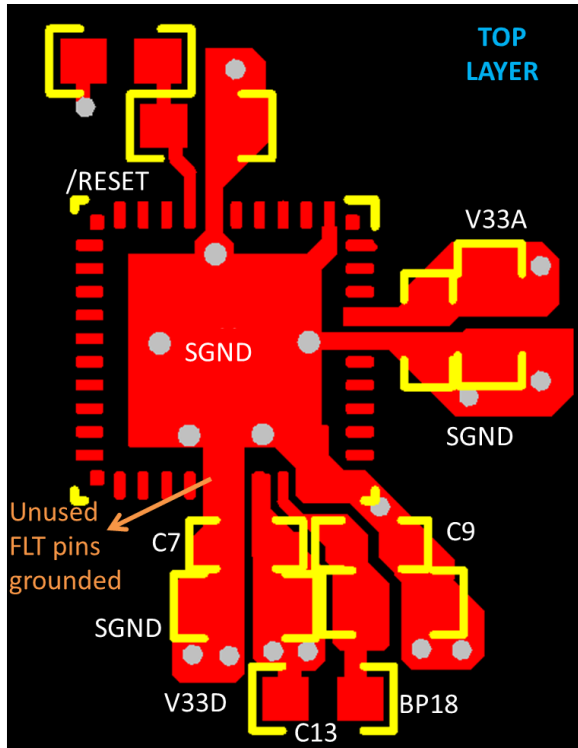
12-11. UCD3138 and UCD3138064 40 Pin Layout Top Layer
