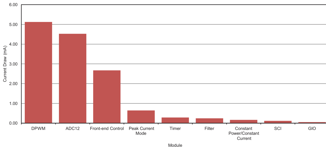
8-4. Clock Gating Power Savings
