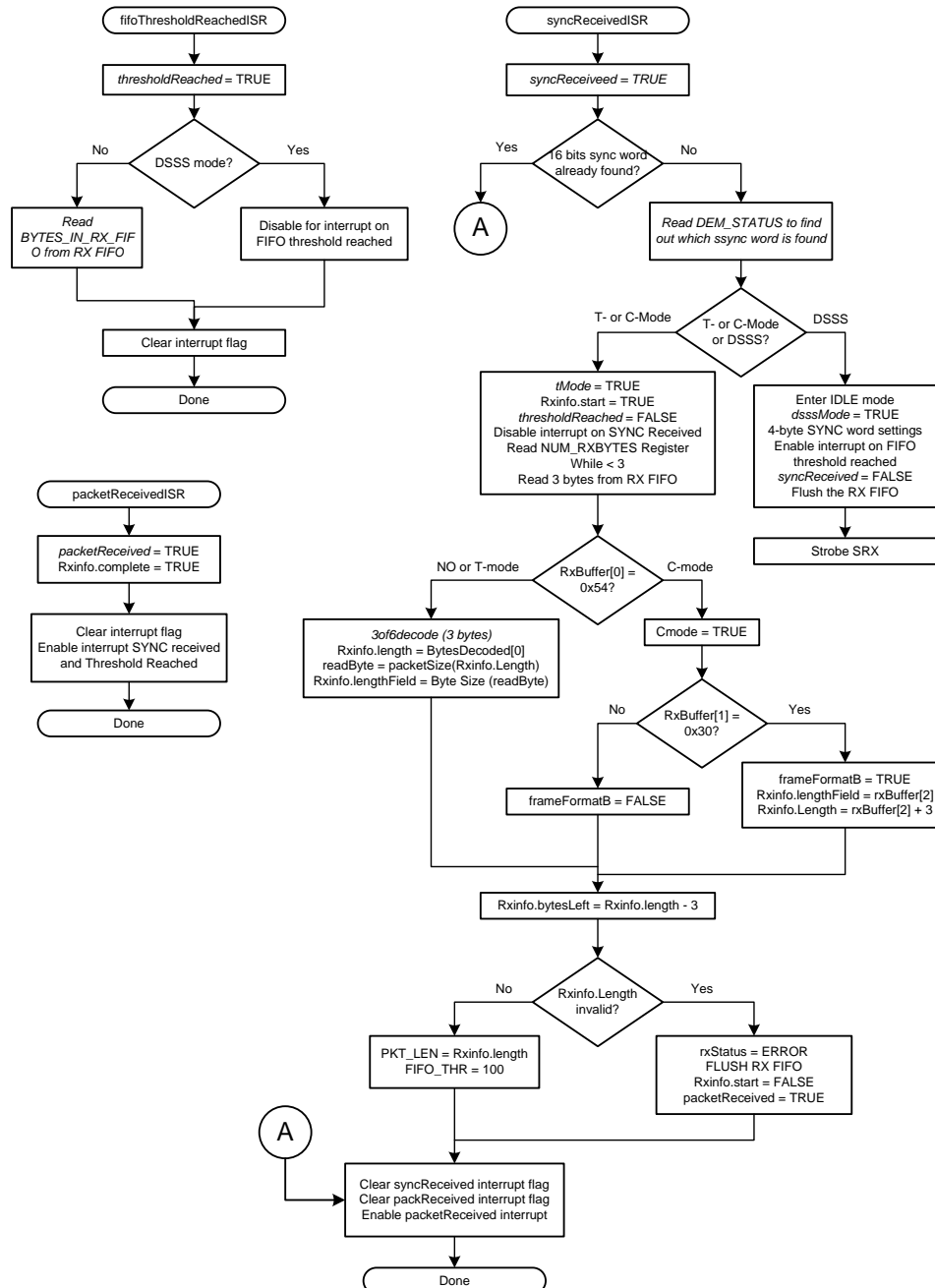
Figure 9. Flow Chart of Interrupt Functions in TIDC-DSSS868WMBUS-DC Firmware
