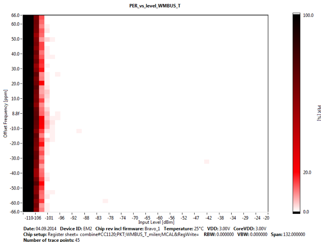
Figure 12. T-Mode Receive Operation With CC1125 With 10-Byte Payload, 100 kcps, 2-FSK, and Frequency = 868.95 MHz
