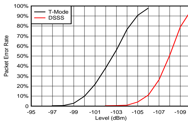
Figure 13. RX Sensitivity Comparison for DSSS-coded Mode With 15.5 Bytes versus wM-Bus T-Mode With 20 Bytes
