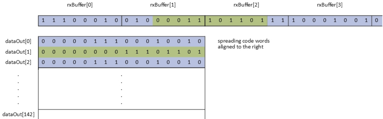
Figure 10. dataOut[] Buffer Filled Up With 11-Bit Spreading Sequence
