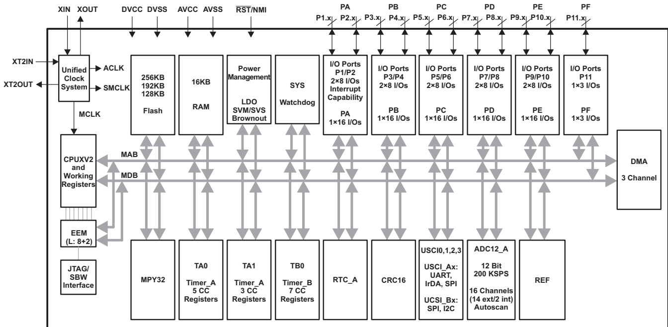
Figure 1. MSP430F5438A Functional Block Diagram
