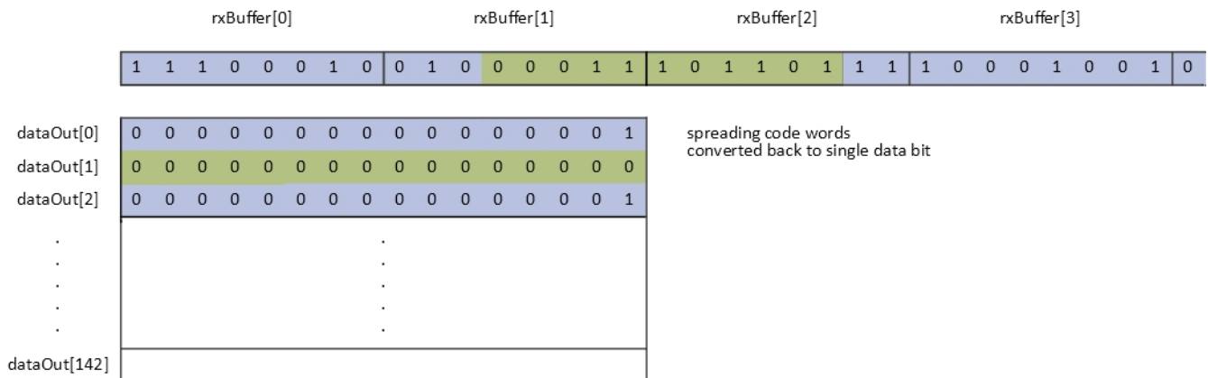
Figure 11. dataOut[] Buffer Converted into “0” or “1” for all 142 Groups
