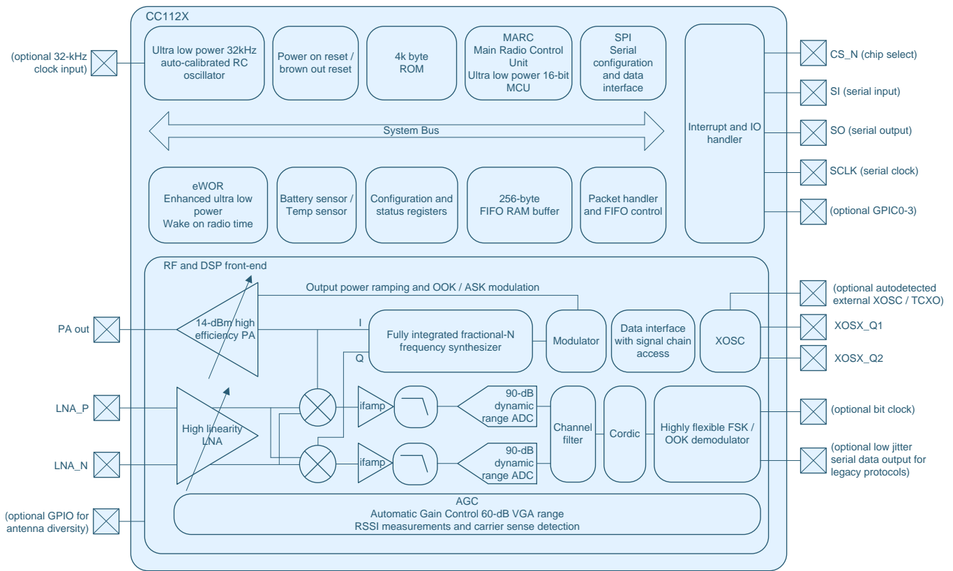
図 2. CC1125 Functional Block Diagram
