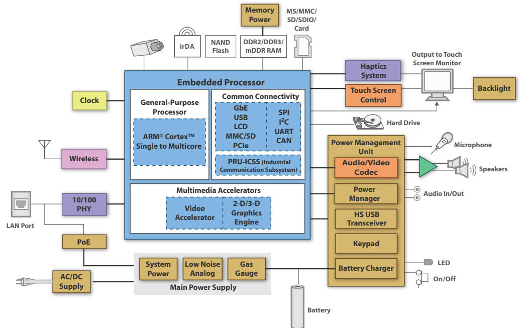
HMI system block diagram of mid to high end system
