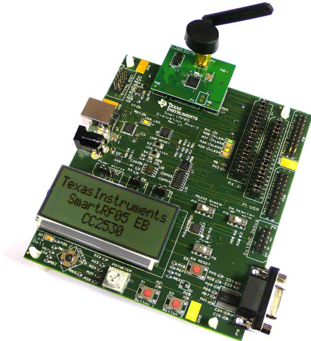
Figure 1 SmartRF05EB with CC2530EM
