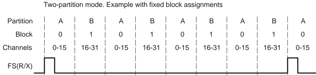
Figure 5-1. Alternating Between the Channels of Partition A and the Channels of Partition B
