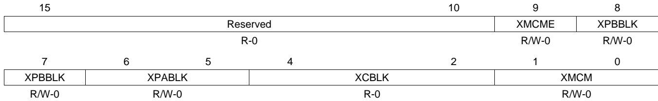
Figure 11-12. Multichannel Control 2 Register (MCR2)
