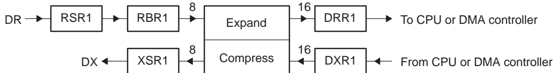
Figure 8-3. Companding Processes for Reception and for Transmission
