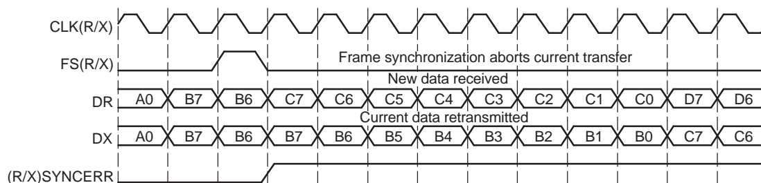
Figure 7-1. Unexpected Frame-Synchronization Pulse With (R/X)FIG = 0
