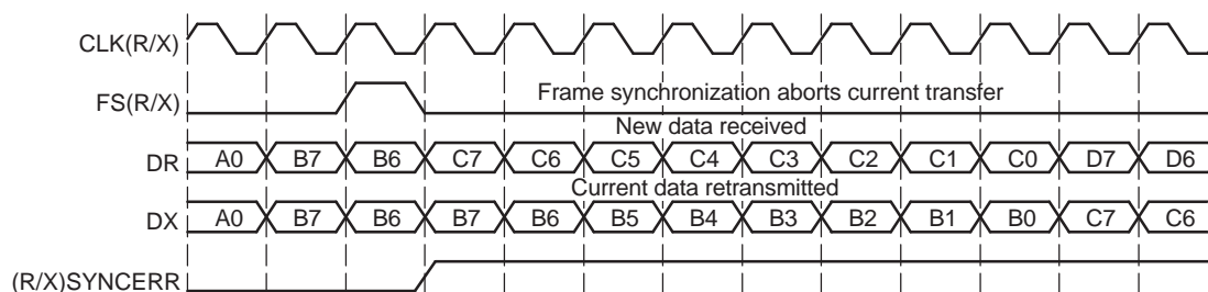
Figure 8-1. Unexpected Frame-Synchronization Pulse With (R/X) FIG = 0
