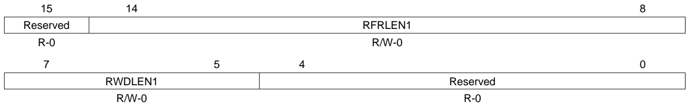
Figure 11-5. Receive Control Register 1 (RCR1)
