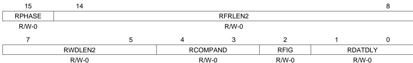
Figure 11-6. Receive Control Register 2 (RCR2)
