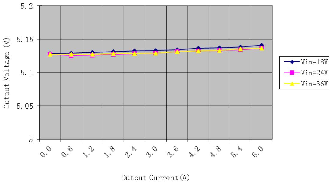
Load Regulation
