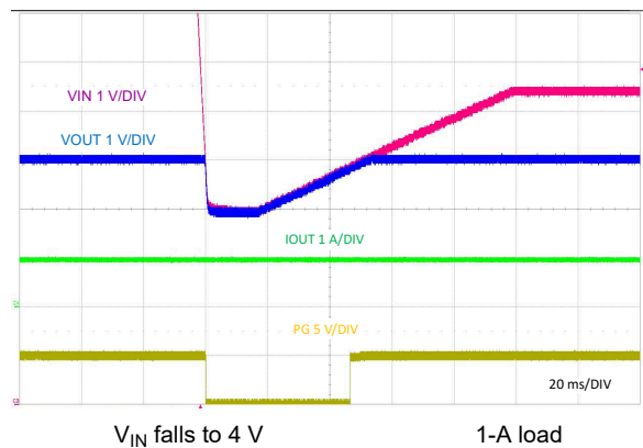
Figure 9-24. Line Transient Response to V_{IN} = 4 V
