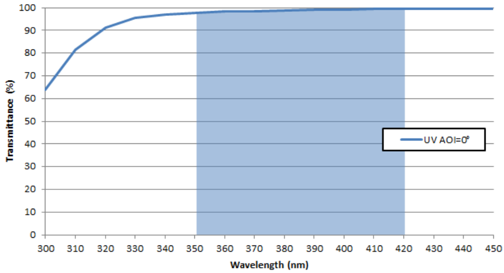
Figure 3. Corning 7056 UV Window Transmittance (UV Region)
